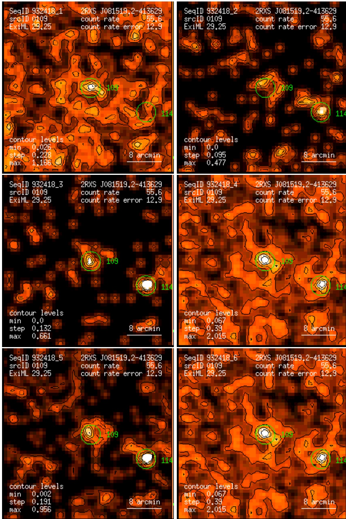
Figure 109: RASS 932418: detection 0109: band rate images, Gaussian filter: (1) PSPC channels 11 – 41, (2) 52 – 90, (3) 91 – 201, (4) 11 – 235, (5) 52 – 201, (6) 11 – 201. Broad band rates in counts/ks. Band rate contour levels in counts/ks/arcmin 2 .
