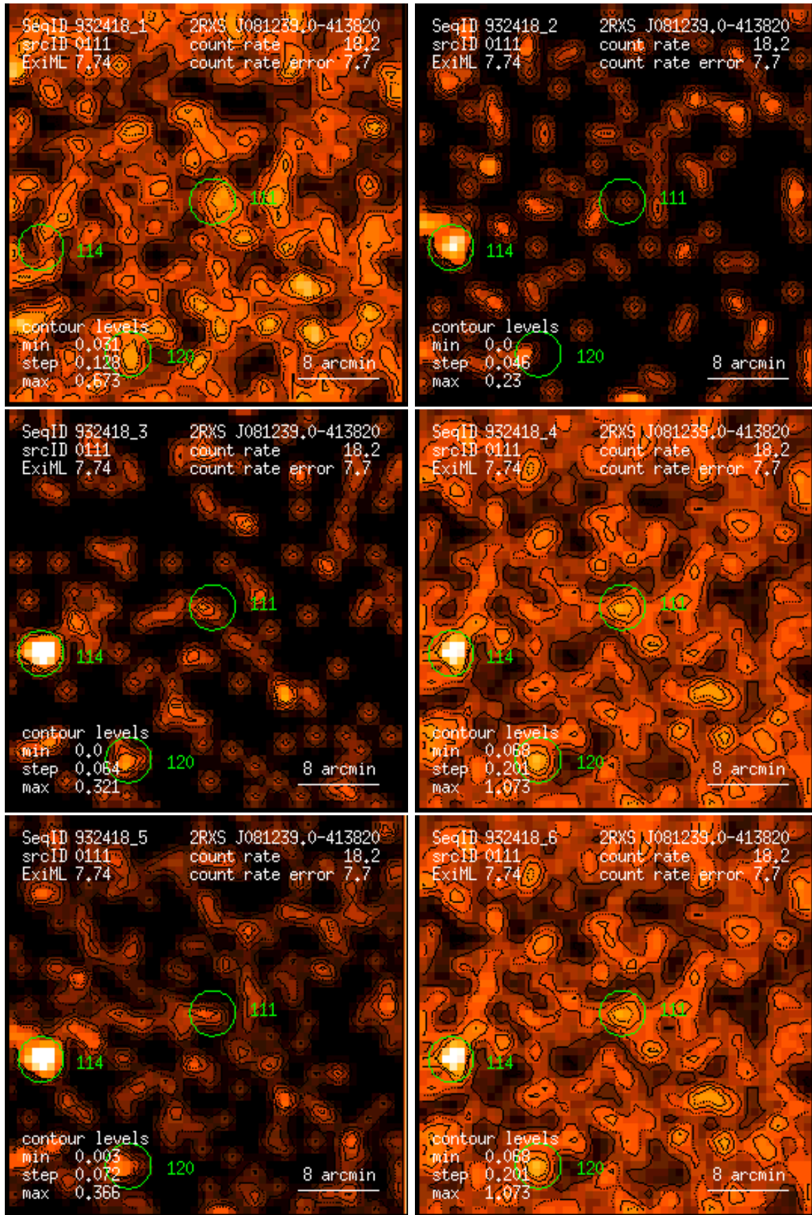
Figure 111: RASS 932418: detection 0111: band rate images, Gaussian filter: (1) PSPC channels 11 – 41, (2) 52 – 90, (3) 91 – 201, (4) 11 – 235, (5) 52 – 201, (6) 11 – 201. Broad band rates in counts/ks. Band rate contour levels in counts/ks/arcmin 2 .
