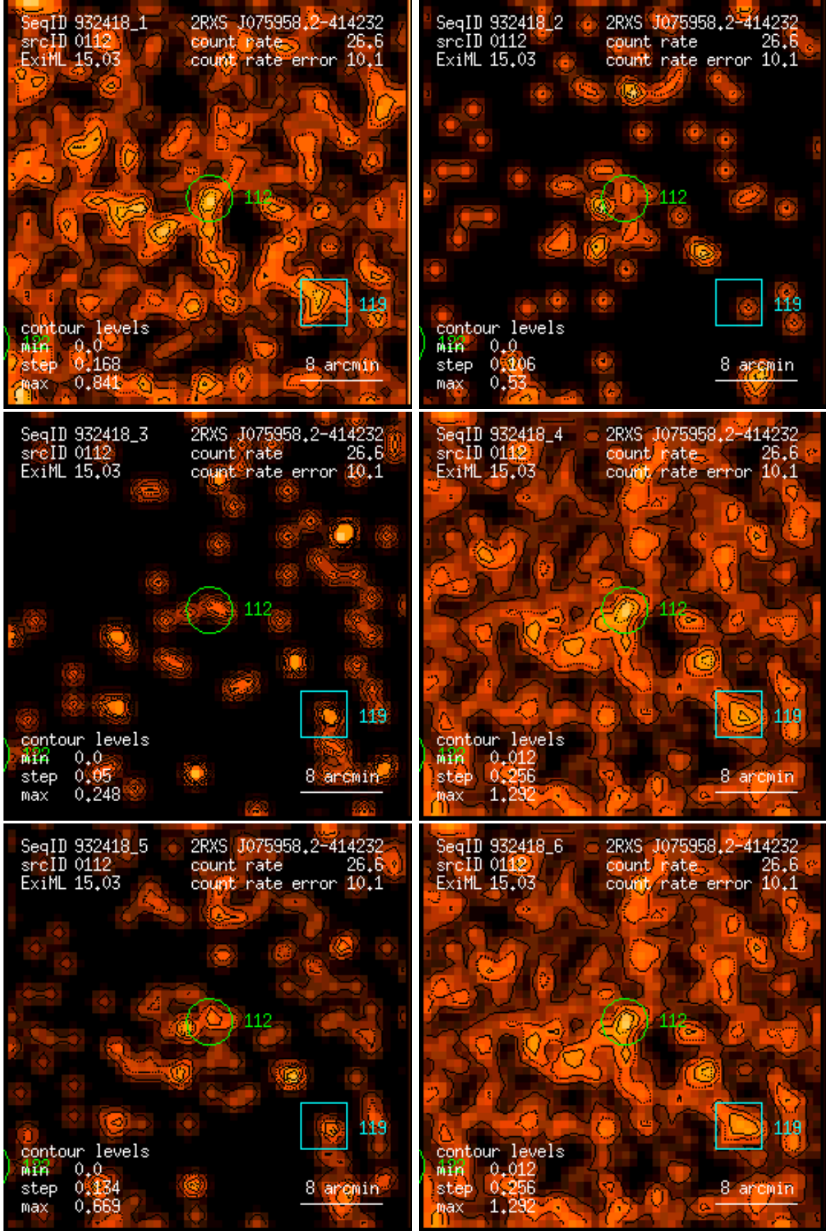
Figure 112: RASS 932418: detection 0112: band rate images, Gaussian filter: (1) PSPC channels 11 – 41, (2) 52 – 90, (3) 91 – 201, (4) 11 – 235, (5) 52 – 201, (6) 11 – 201. Broad band rates in counts/ks. Band rate contour levels in counts/ks/arcmin 2 .
