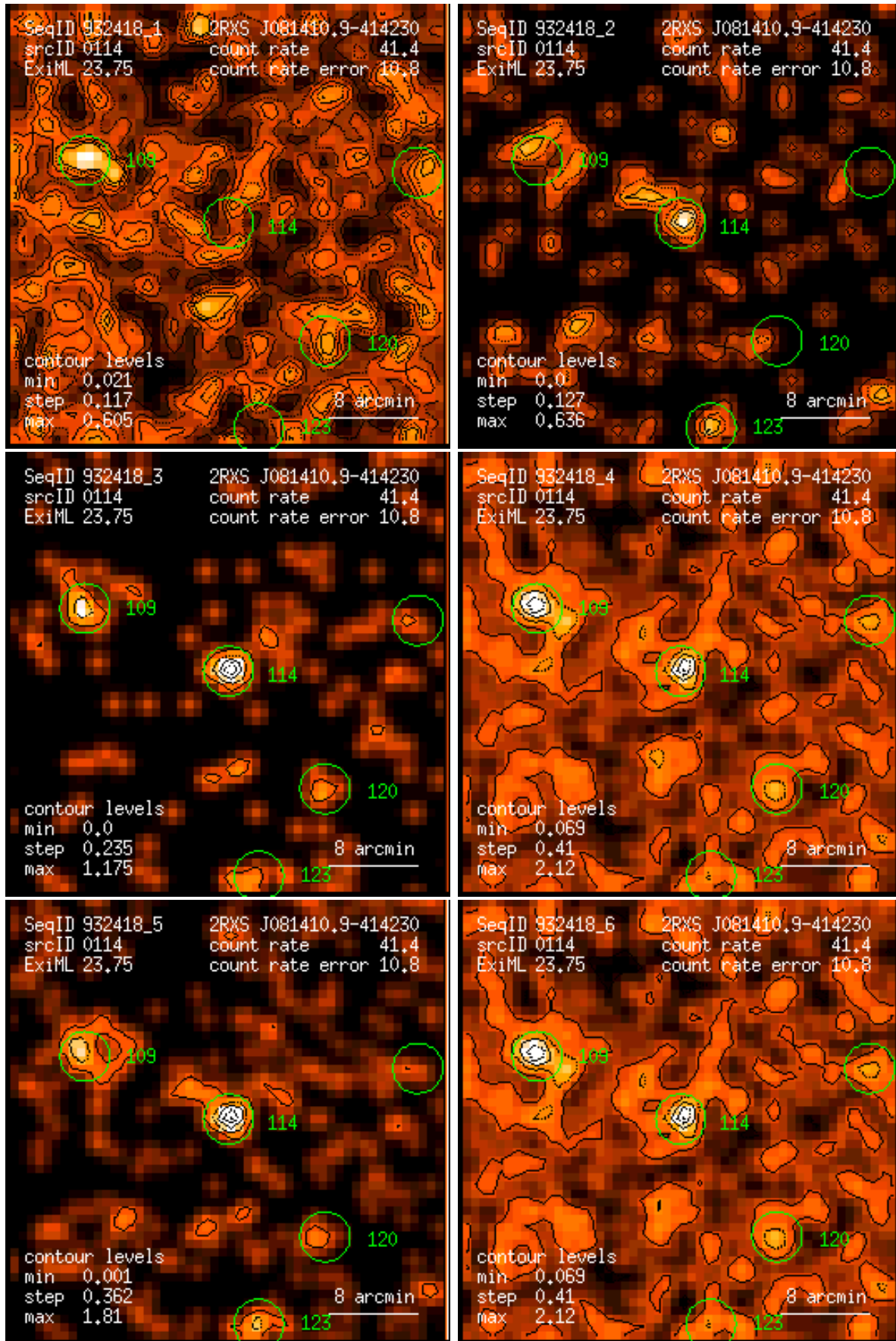
Figure 114: RASS 932418: detection 0114: band rate images, Gaussian filter: (1) PSPC channels 11 – 41, (2) 52 – 90, (3) 91 – 201, (4) 11 – 235, (5) 52 – 201, (6) 11 – 201. Broad band rates in counts/ks. Band rate contour levels in counts/ks/arcmin 2 .
