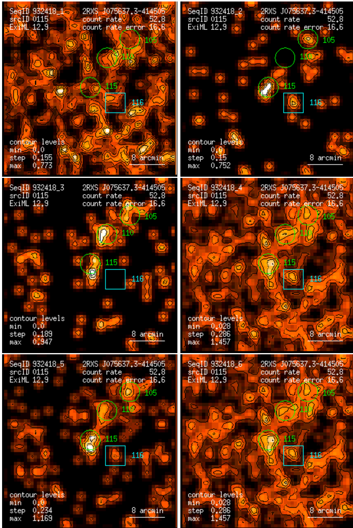
Figure 115: RASS 932418: detection 0115: band rate images, Gaussian filter: (1) PSPC channels 11 – 41, (2) 52 – 90, (3) 91 – 201, (4) 11 – 235, (5) 52 – 201, (6) 11 – 201. Broad band rates in counts/ks. Band rate contour levels in counts/ks/arcmin 2 .
