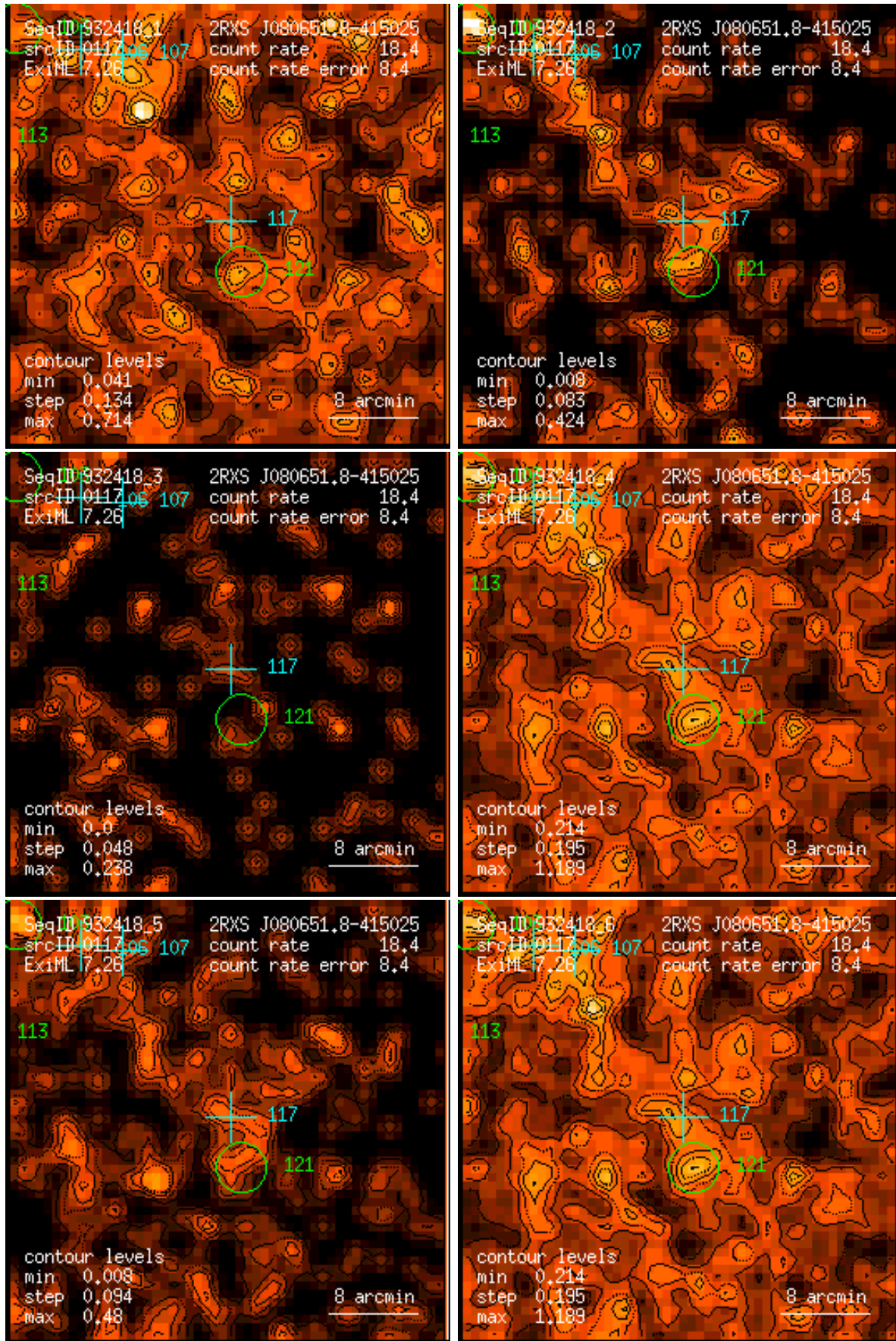
Figure 117: RASS 932418: detection 0117: band rate images, Gaussian filter: (1) PSPC channels 11 – 41, (2) 52 – 90, (3) 91 – 201, (4) 11 – 235, (5) 52 – 201, (6) 11 – 201. Broad band rates in counts/ks. Band rate contour levels in counts/ks/arcmin 2 .
