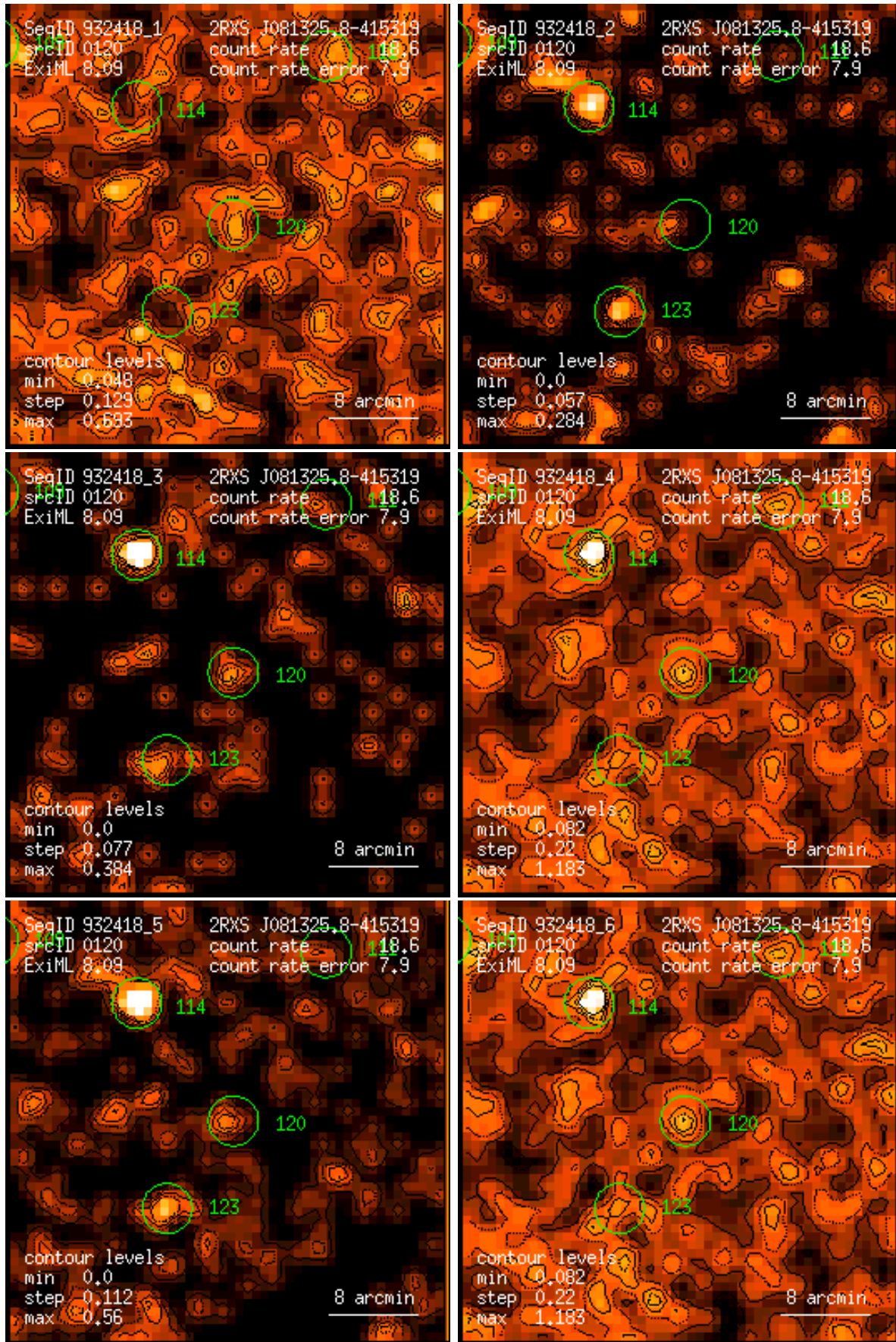
Figure 120: RASS 932418: detection 0120: band rate images, Gaussian filter: (1) PSPC channels 11 – 41, (2) 52 – 90, (3) 91 – 201, (4) 11 – 235, (5) 52 – 201, (6) 11 – 201. Broad band rates in counts/ks. Band rate contour levels in counts/ks/arcmin 2 .
