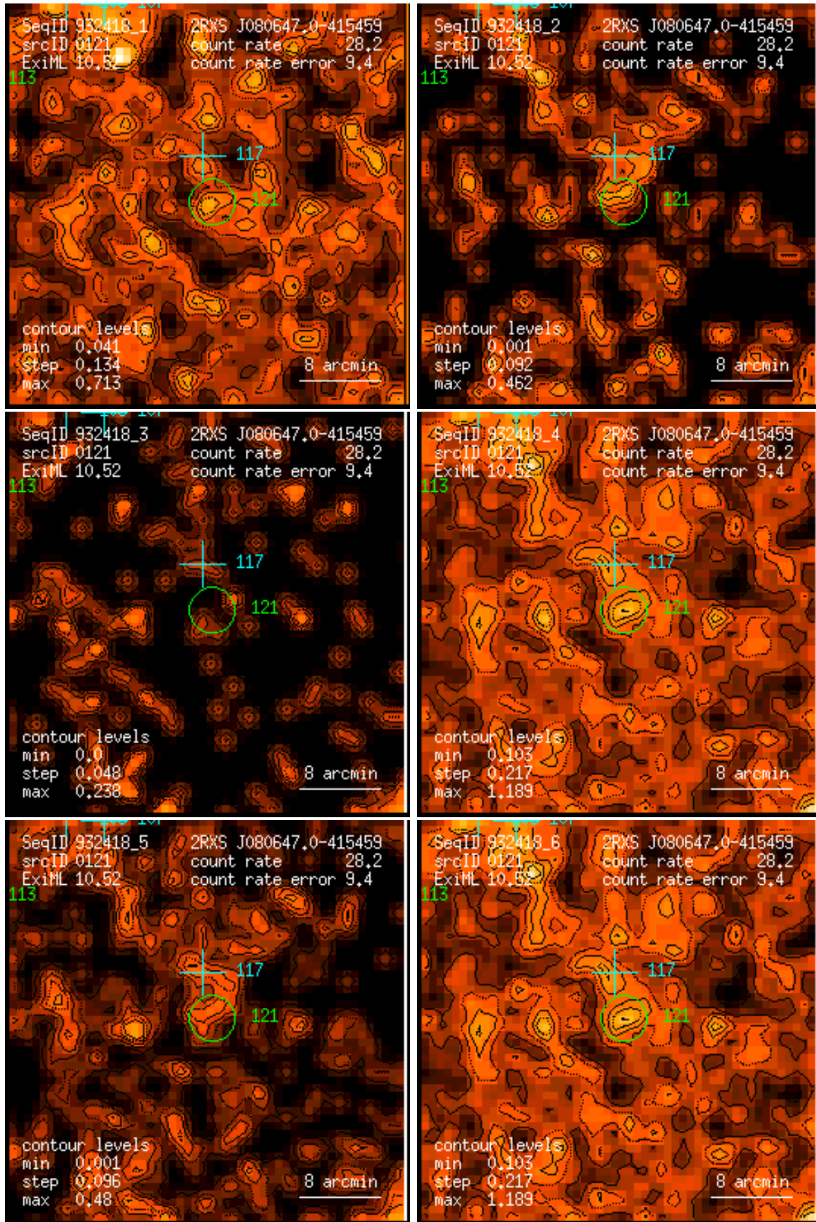
Figure 121: RASS 932418: detection 0121: band rate images, Gaussian filter: (1) PSPC channels 11 – 41, (2) 52 – 90, (3) 91 – 201, (4) 11 – 235, (5) 52 – 201, (6) 11 – 201. Broad band rates in counts/ks. Band rate contour levels in counts/ks/arcmin 2 .
