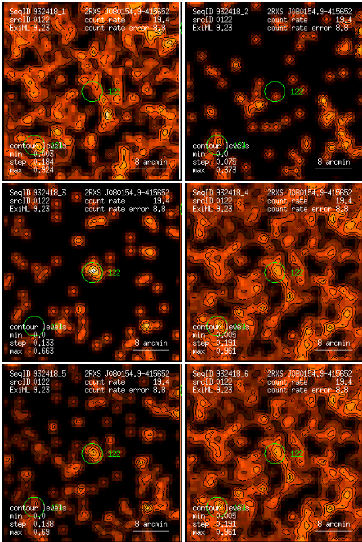
Figure 122: RASS 932418: detection 0122: band rate images, Gaussian filter: (1) PSPC channels 11 – 41, (2) 52 – 90, (3) 91 – 201, (4) 11 – 235, (5) 52 – 201, (6) 11 – 201. Broad band rates in counts/ks. Band rate contour levels in counts/ks/arcmin 2 .
