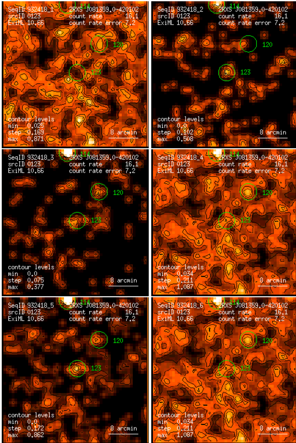
Figure 123: RASS 932418: detection 0123: band rate images, Gaussian filter: (1) PSPC channels 11 – 41, (2) 52 – 90, (3) 91 – 201, (4) 11 – 235, (5) 52 – 201, (6) 11 – 201. Broad band rates in counts/ks. Band rate contour levels in counts/ks/arcmin 2 .
