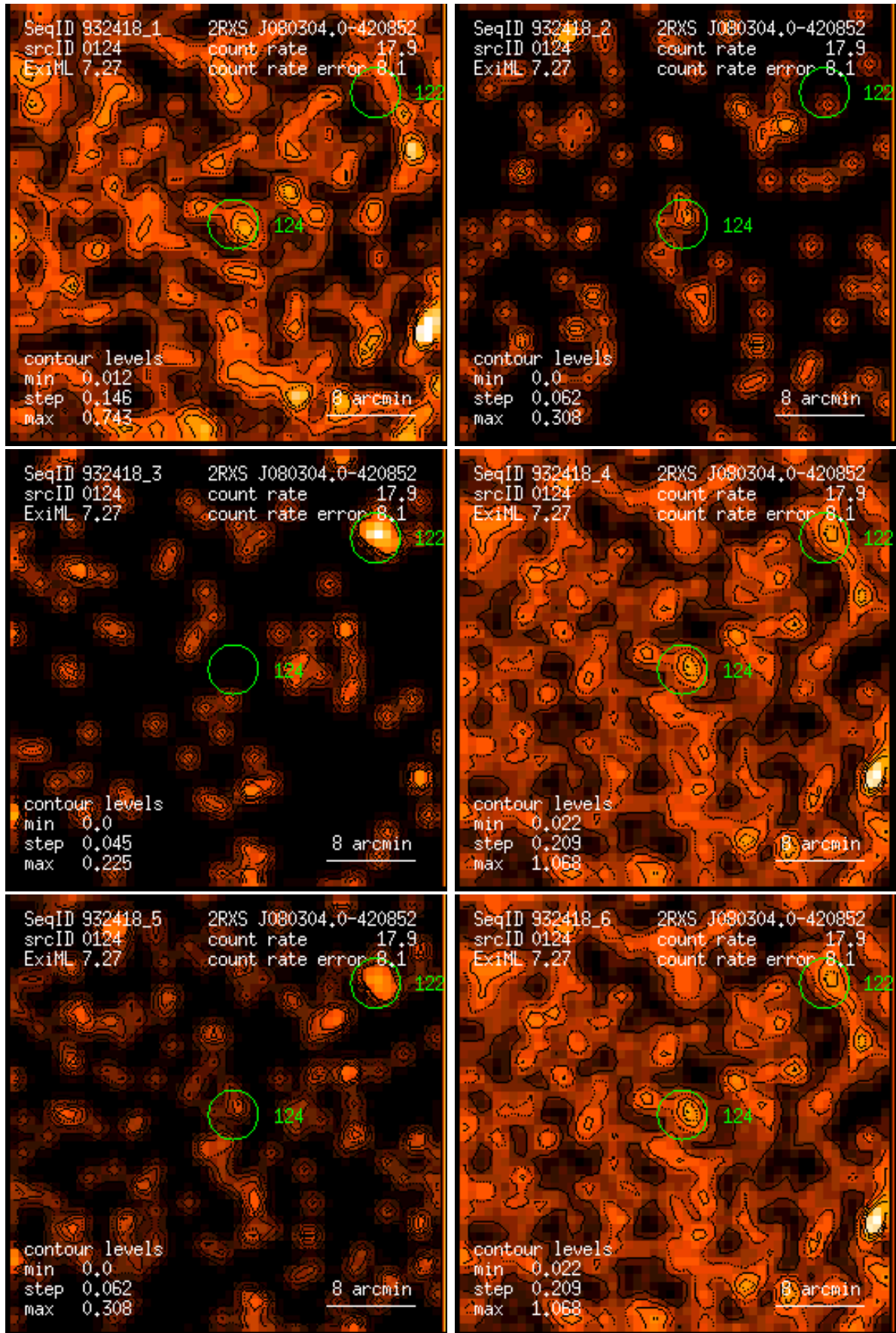
Figure 124: RASS 932418: detection 0124: band rate images, Gaussian filter: (1) PSPC channels 11 – 41, (2) 52 – 90, (3) 91 – 201, (4) 11 – 235, (5) 52 – 201, (6) 11 – 201. Broad band rates in counts/ks. Band rate contour levels in counts/ks/arcmin 2 .
