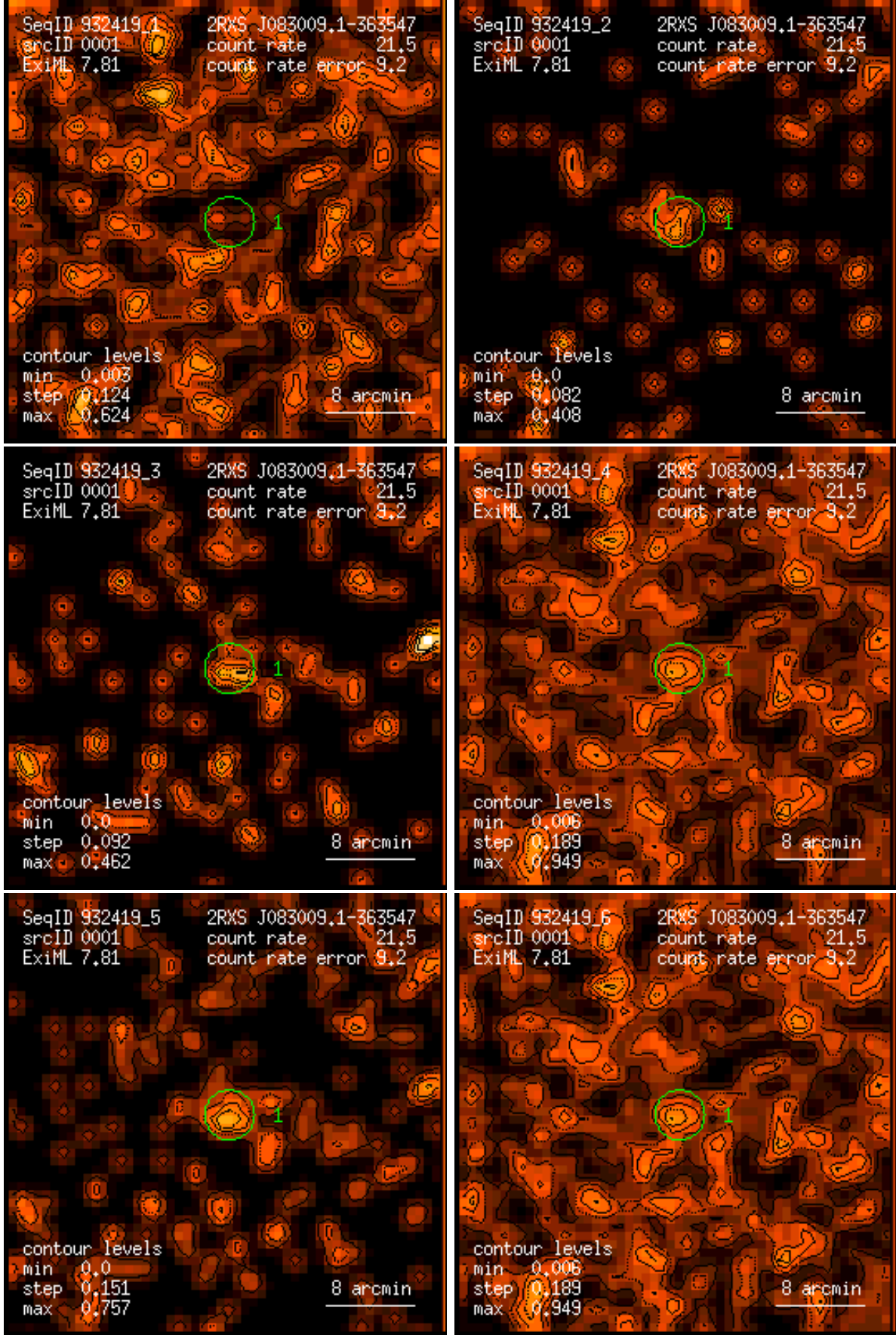
Figure 1: RASS 932419: detection 0001: band rate images, Gaussian filter: (1) PSPC channels 11 – 41, (2) 52 – 90, (3) 91 – 201, (4) 11 – 235, (5) 52 – 201, (6) 11 – 201. Broad band rates in counts/ks. Band rate contour levels in counts/ks/arcmin 2 .
