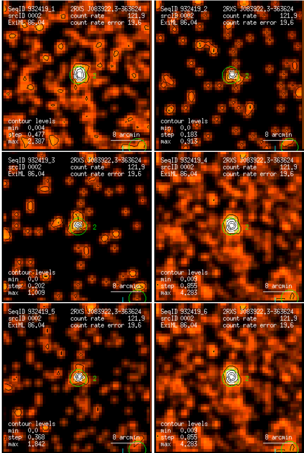
Figure 2: RASS 932419: detection 0002: band rate images, Gaussian filter: (1) PSPC channels 11 – 41, (2) 52 – 90, (3) 91 – 201, (4) 11 – 235, (5) 52 – 201, (6) 11 – 201. Broad band rates in counts/ks. Band rate contour levels in counts/ks/arcmin 2 .
