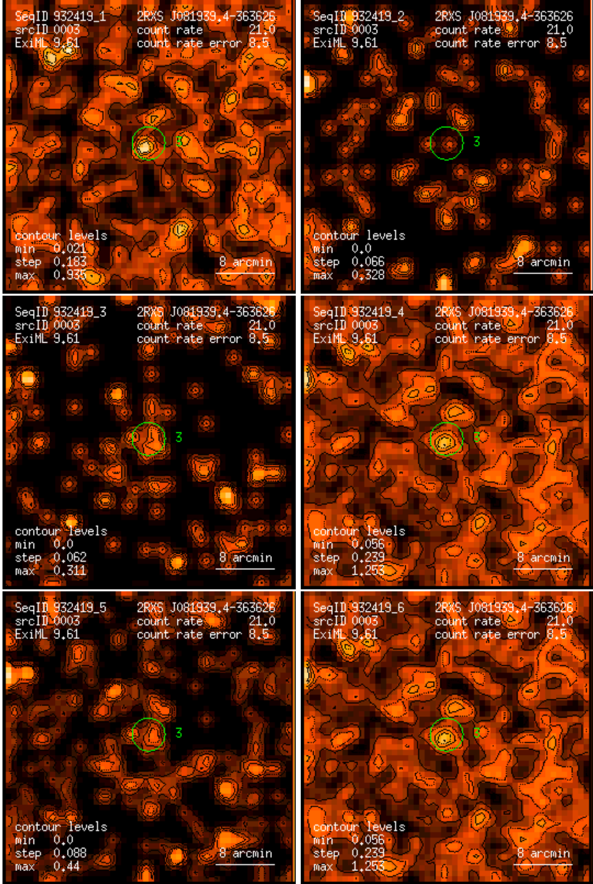
Figure 3: RASS 932419: detection 0003: band rate images, Gaussian filter: (1) PSPC channels 11 – 41, (2) 52 – 90, (3) 91 – 201, (4) 11 – 235, (5) 52 – 201, (6) 11 – 201. Broad band rates in counts/ks. Band rate contour levels in counts/ks/arcmin 2 .
