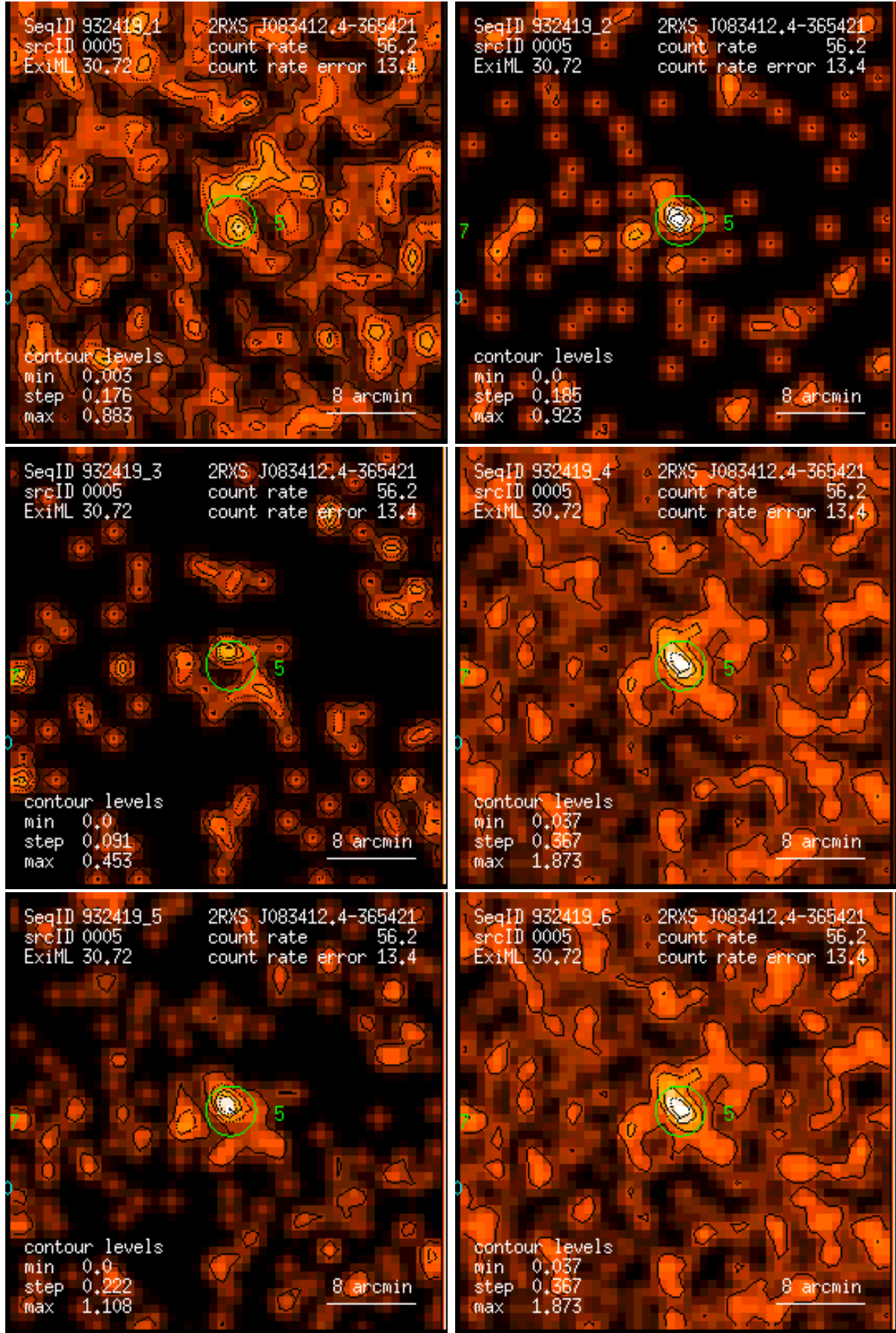
Figure 5: RASS 932419: detection 0005: band rate images, Gaussian filter: (1) PSPC channels 11 – 41, (2) 52 – 90, (3) 91 – 201, (4) 11 – 235, (5) 52 – 201, (6) 11 – 201. Broad band rates in counts/ks. Band rate contour levels in counts/ks/arcmin 2 .
