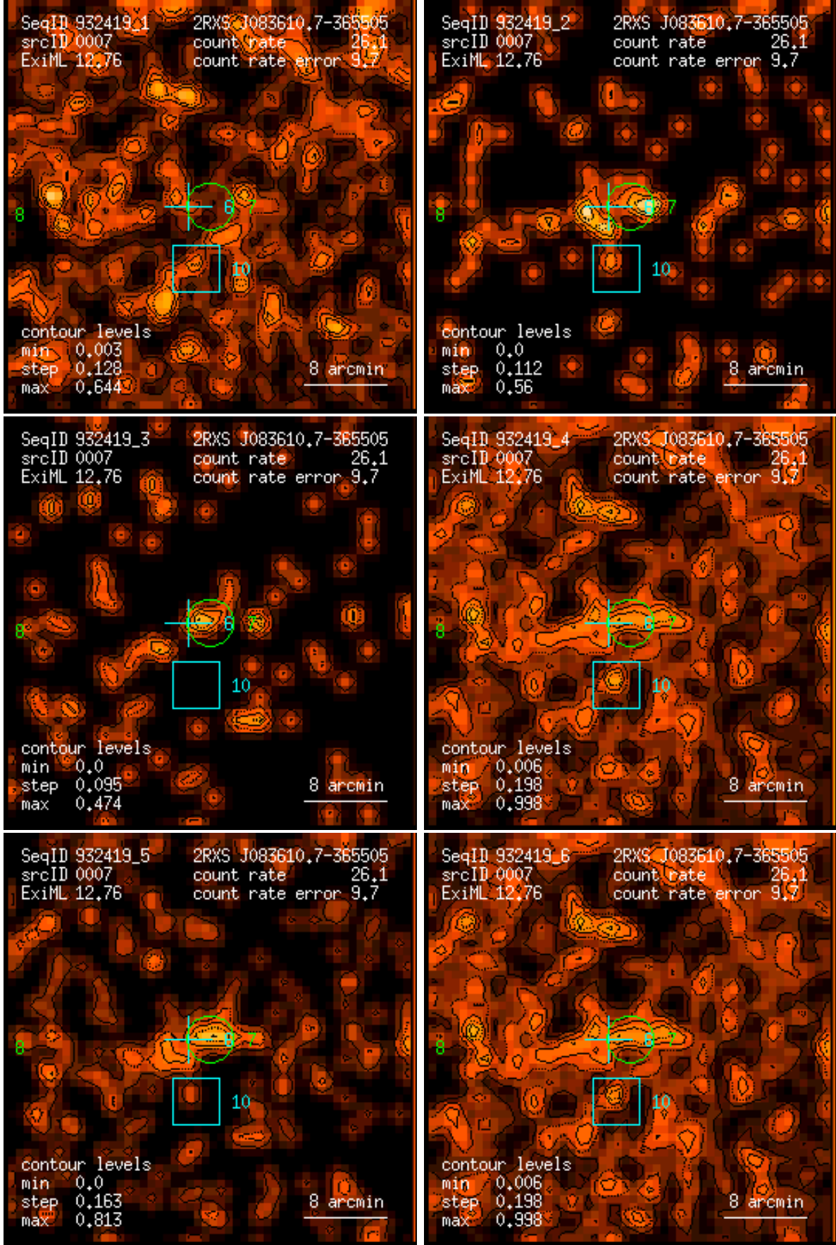
Figure 7: RASS 932419: detection 0007: band rate images, Gaussian filter: (1) PSPC channels 11 – 41, (2) 52 – 90, (3) 91 – 201, (4) 11 – 235, (5) 52 – 201, (6) 11 – 201. Broad band rates in counts/ks. Band rate contour levels in counts/ks/arcmin 2 .
