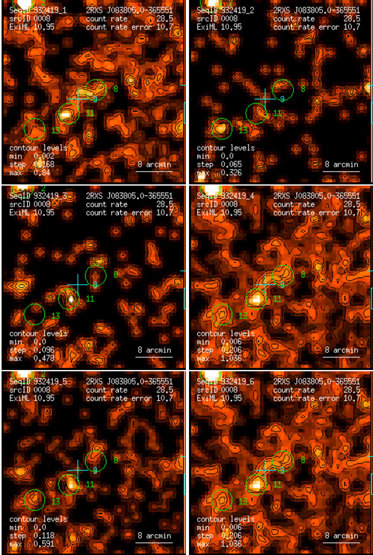
Figure 8: RASS 932419: detection 0008: band rate images, Gaussian filter: (1) PSPC channels 11 – 41, (2) 52 – 90, (3) 91 – 201, (4) 11 – 235, (5) 52 – 201, (6) 11 – 201. Broad band rates in counts/ks. Band rate contour levels in counts/ks/arcmin 2 .
