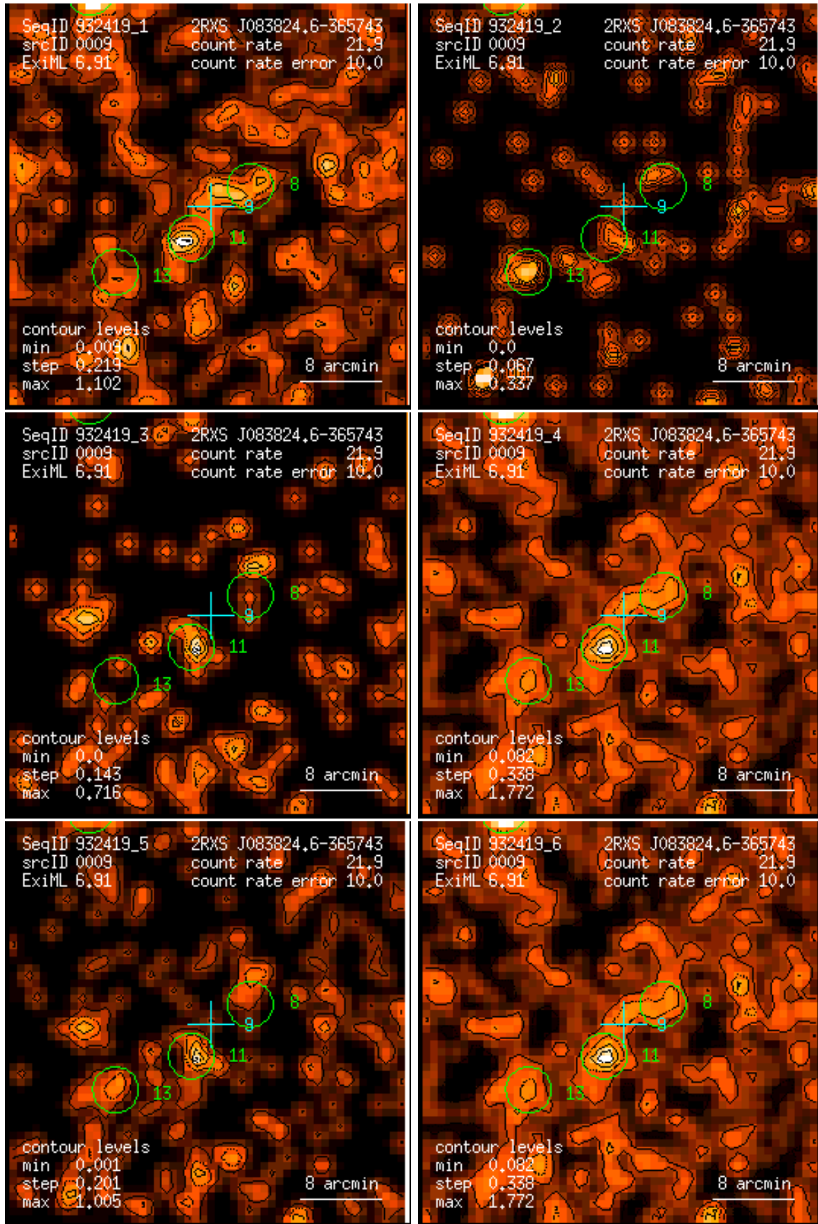
Figure 9: RASS 932419: detection 0009: band rate images, Gaussian filter: (1) PSPC channels 11 – 41, (2) 52 – 90, (3) 91 – 201, (4) 11 – 235, (5) 52 – 201, (6) 11 – 201. Broad band rates in counts/ks. Band rate contour levels in counts/ks/arcmin 2 .
