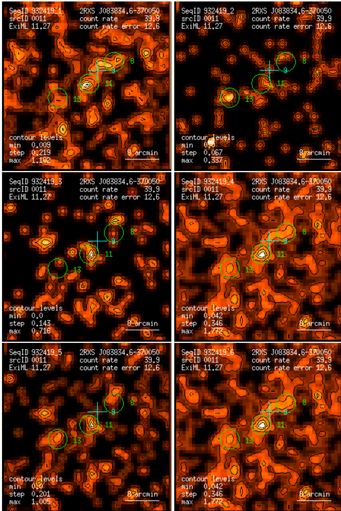
Figure 11: RASS 932419: detection 0011: band rate images, Gaussian filter: (1) PSPC channels 11 – 41, (2) 52 – 90, (3) 91 – 201, (4) 11 – 235, (5) 52 – 201, (6) 11 – 201. Broad band rates in counts/ks. Band rate contour levels in counts/ks/arcmin 2 .
