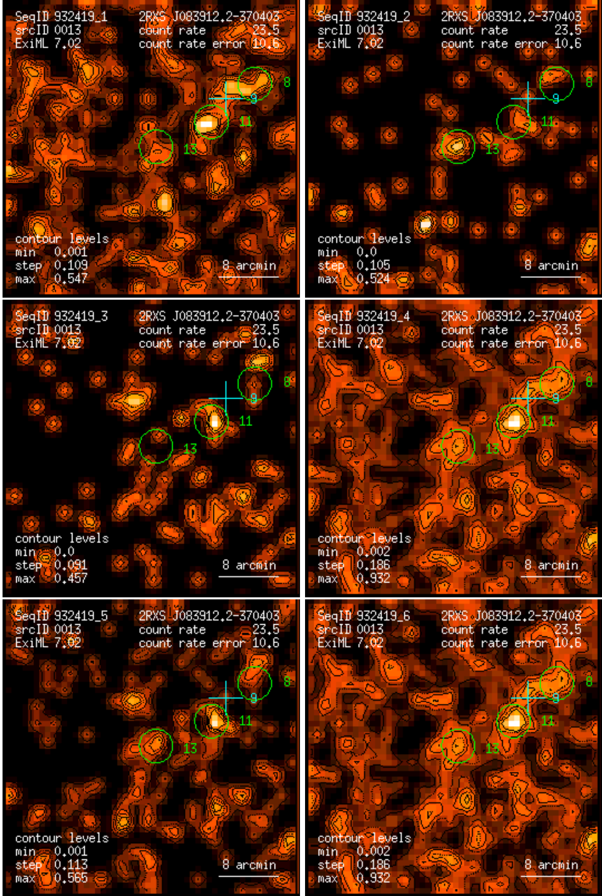
Figure 13: RASS 932419: detection 0013: band rate images, Gaussian filter: (1) PSPC channels 11 – 41, (2) 52 – 90, (3) 91 – 201, (4) 11 – 235, (5) 52 – 201, (6) 11 – 201. Broad band rates in counts/ks. Band rate contour levels in counts/ks/arcmin 2 .
