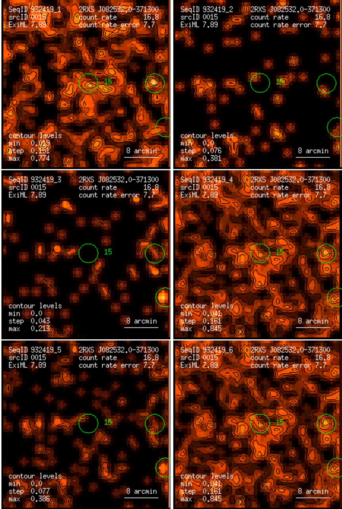
Figure 15: RASS 932419: detection 0015: band rate images, Gaussian filter: (1) PSPC channels 11 – 41, (2) 52 – 90, (3) 91 – 201, (4) 11 – 235, (5) 52 – 201, (6) 11 – 201. Broad band rates in counts/ks. Band rate contour levels in counts/ks/arcmin 2 .
