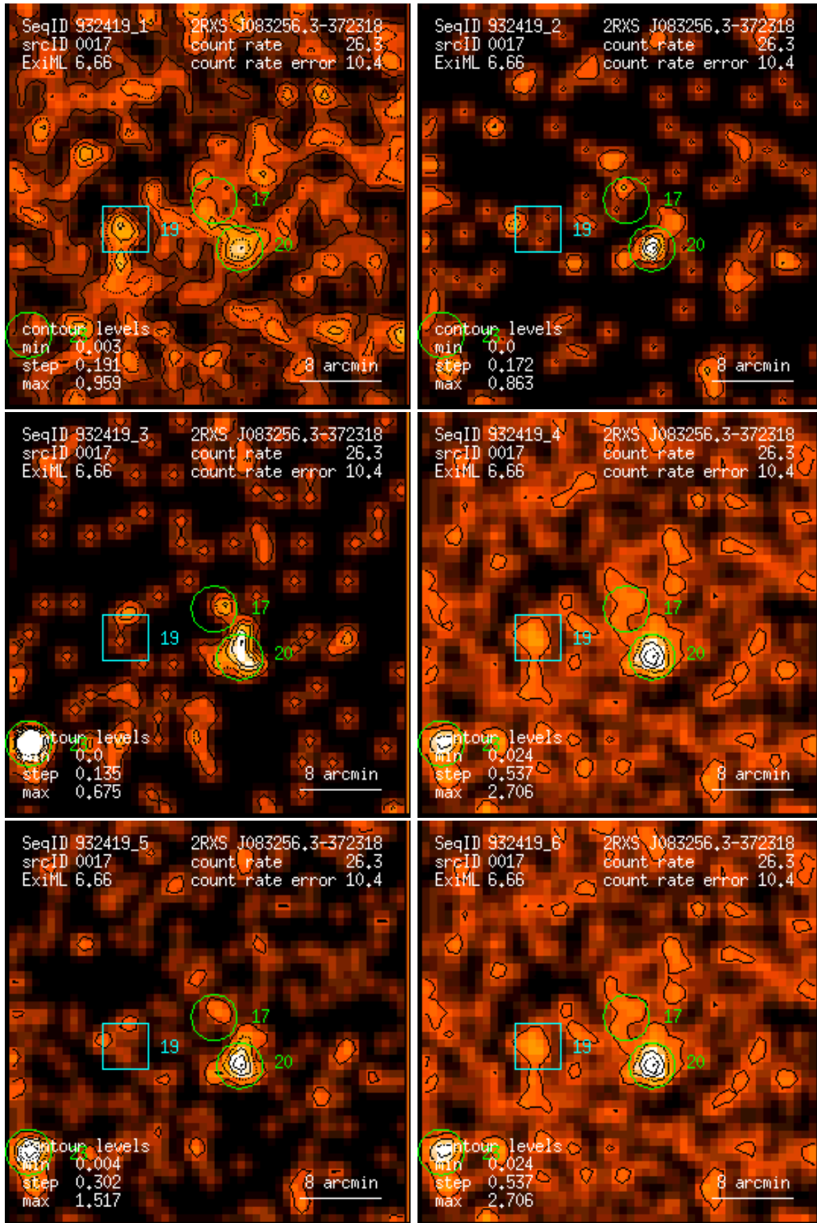
Figure 17: RASS 932419: detection 0017: band rate images, Gaussian filter: (1) PSPC channels 11 – 41, (2) 52 – 90, (3) 91 – 201, (4) 11 – 235, (5) 52 – 201, (6) 11 – 201. Broad band rates in counts/ks. Band rate contour levels in counts/ks/arcmin 2 .
