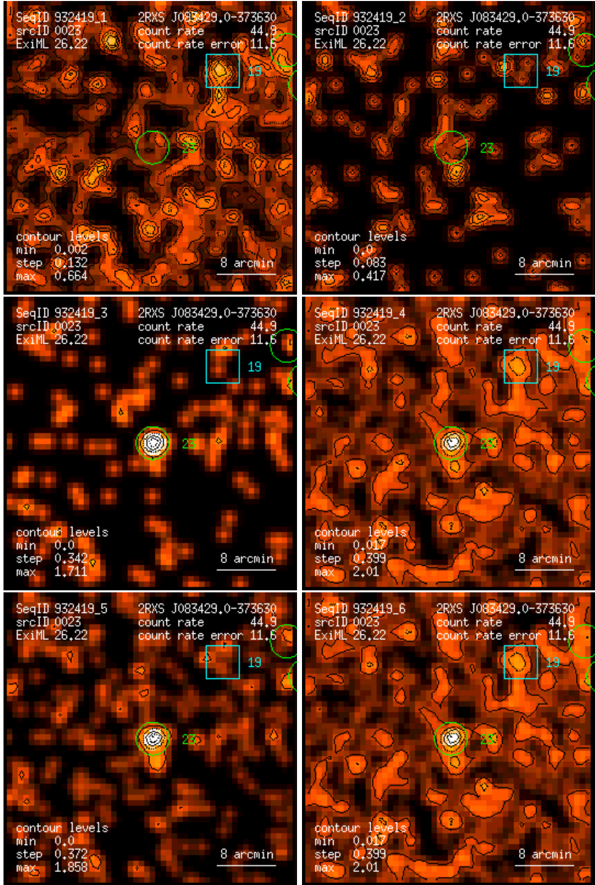
Figure 23: RASS 932419: detection 0023: band rate images, Gaussian filter: (1) PSPC channels 11 – 41, (2) 52 – 90, (3) 91 – 201, (4) 11 – 235, (5) 52 – 201, (6) 11 – 201. Broad band rates in counts/ks. Band rate contour levels in counts/ks/arcmin 2 .
