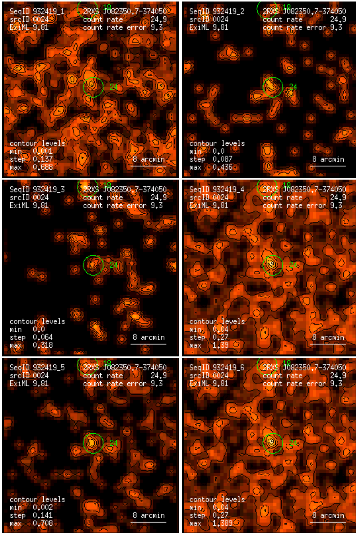
Figure 24: RASS 932419: detection 0024: band rate images, Gaussian filter: (1) PSPC channels 11 – 41, (2) 52 – 90, (3) 91 – 201, (4) 11 – 235, (5) 52 – 201, (6) 11 – 201. Broad band rates in counts/ks. Band rate contour levels in counts/ks/arcmin 2 .
