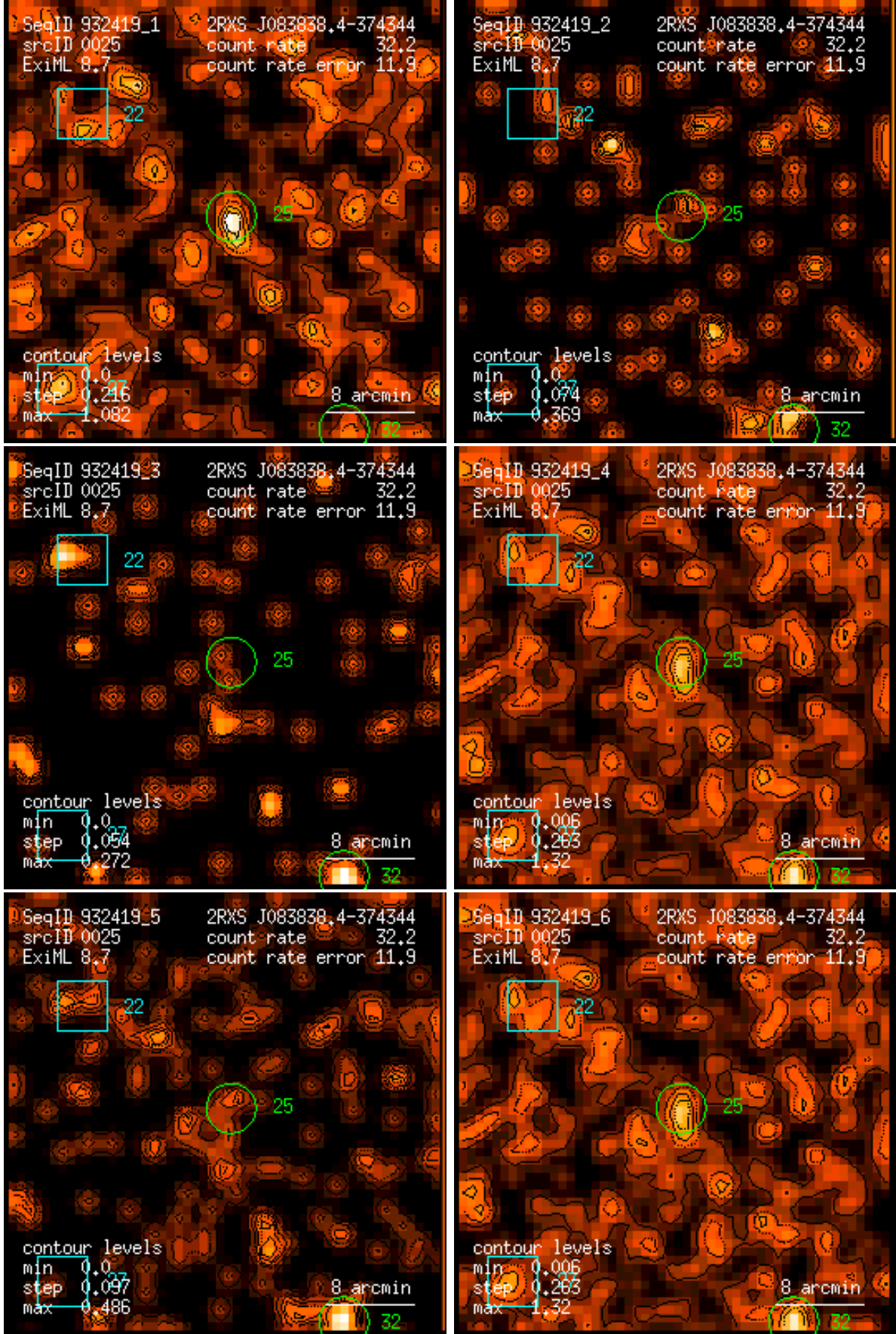
Figure 25: RASS 932419: detection 0025: band rate images, Gaussian filter: (1) PSPC channels 11 – 41, (2) 52 – 90, (3) 91 – 201, (4) 11 – 235, (5) 52 – 201, (6) 11 – 201. Broad band rates in counts/ks. Band rate contour levels in counts/ks/arcmin 2 .
