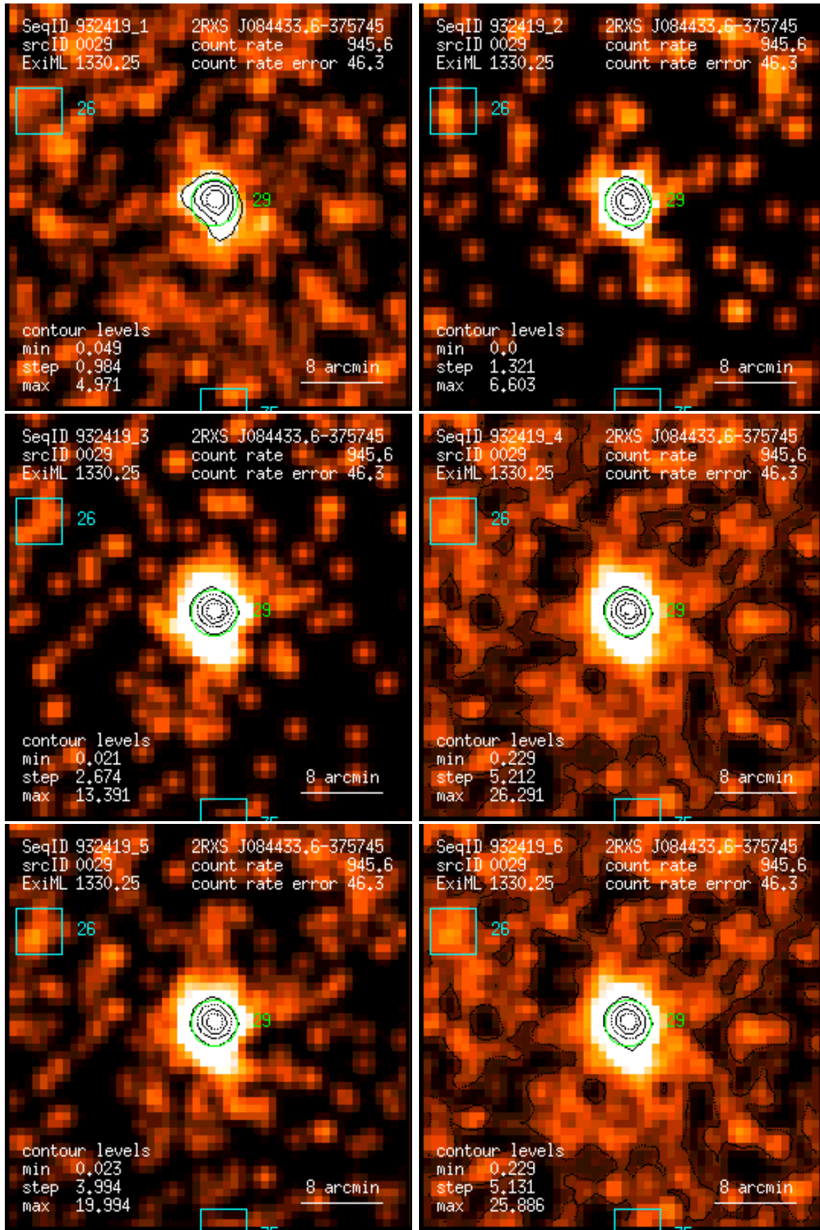
Figure 29: RASS 932419: detection 0029: band rate images, Gaussian filter: (1) PSPC channels 11 – 41, (2) 52 – 90, (3) 91 – 201, (4) 11 – 235, (5) 52 – 201, (6) 11 – 201. Broad band rates in counts/ks. Band rate contour levels in counts/ks/arcmin 2 .
