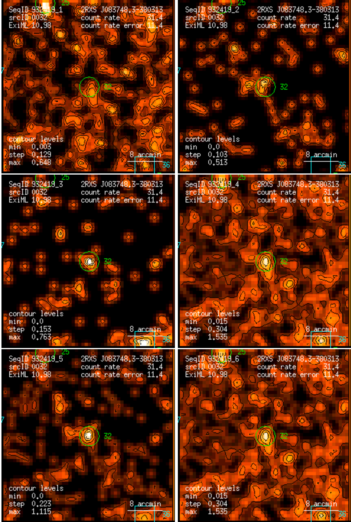
Figure 32: RASS 932419: detection 0032: band rate images, Gaussian filter: (1) PSPC channels 11 – 41, (2) 52 – 90, (3) 91 – 201, (4) 11 – 235, (5) 52 – 201, (6) 11 – 201. Broad band rates in counts/ks. Band rate contour levels in counts/ks/arcmin 2 .
