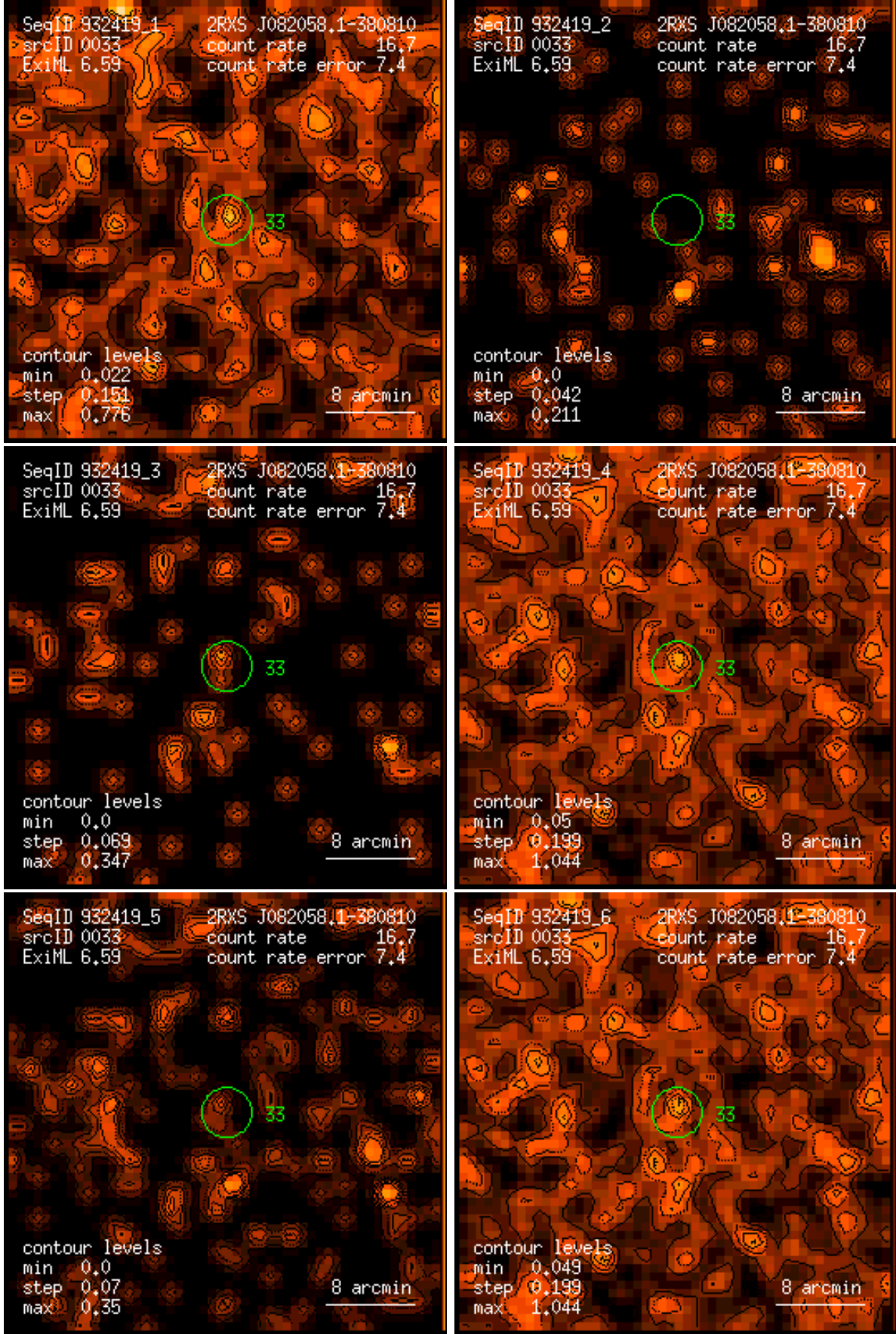
Figure 33: RASS 932419: detection 0033: band rate images, Gaussian filter: (1) PSPC channels 11 – 41, (2) 52 – 90, (3) 91 – 201, (4) 11 – 235, (5) 52 – 201, (6) 11 – 201. Broad band rates in counts/ks. Band rate contour levels in counts/ks/arcmin 2 .
