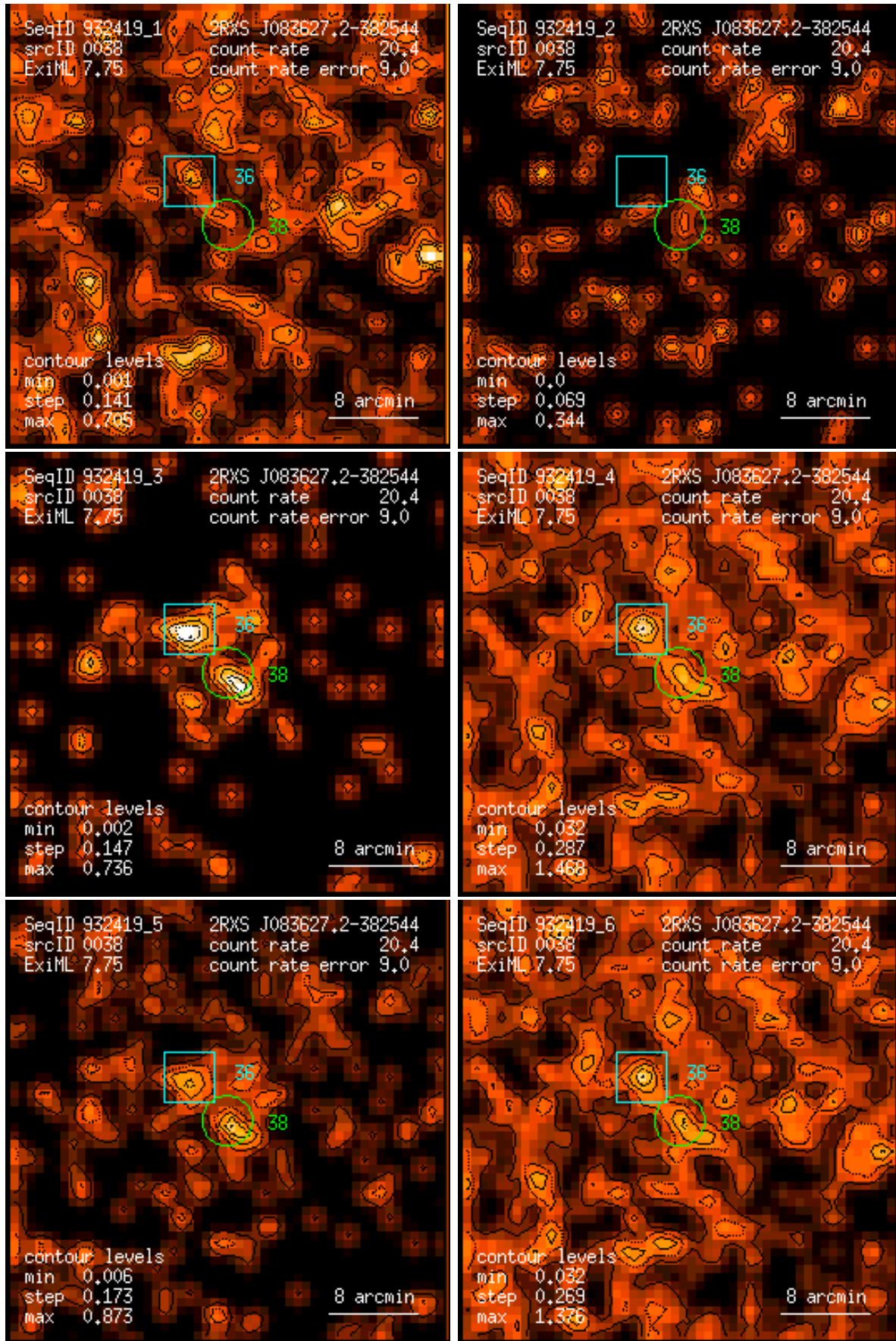
Figure 38: RASS 932419: detection 0038: band rate images, Gaussian filter: (1) PSPC channels 11 – 41, (2) 52 – 90, (3) 91 – 201, (4) 11 – 235, (5) 52 – 201, (6) 11 – 201. Broad band rates in counts/ks. Band rate contour levels in counts/ks/arcmin 2 .
