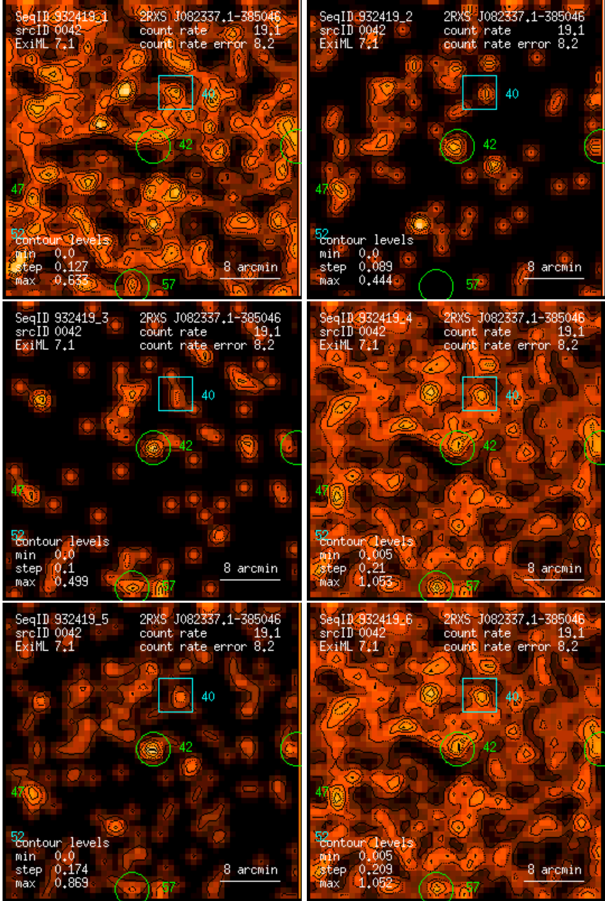
Figure 42: RASS 932419: detection 0042: band rate images, Gaussian filter: (1) PSPC channels 11 – 41, (2) 52 – 90, (3) 91 – 201, (4) 11 – 235, (5) 52 – 201, (6) 11 – 201. Broad band rates in counts/ks. Band rate contour levels in counts/ks/arcmin 2 .
