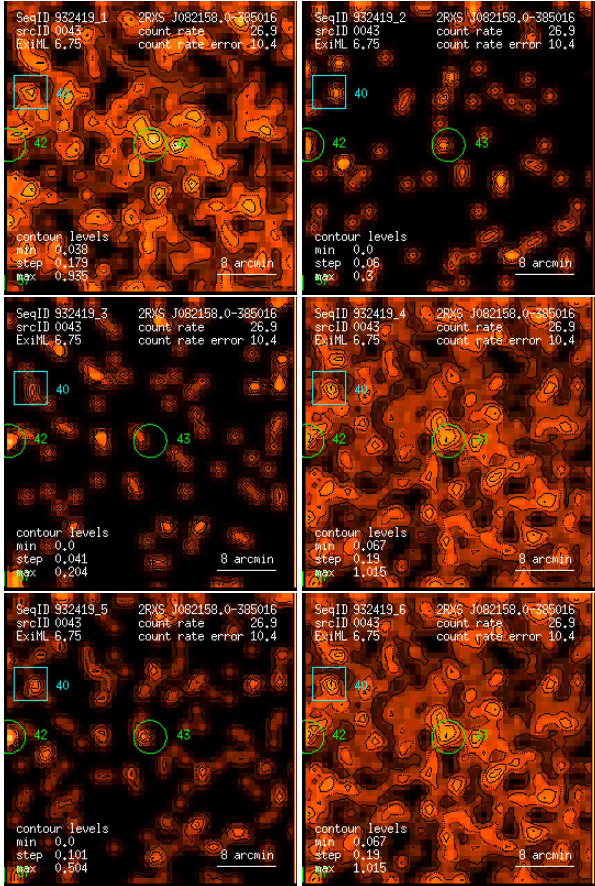
Figure 43: RASS 932419: detection 0043: band rate images, Gaussian filter: (1) PSPC channels 11 – 41, (2) 52 – 90, (3) 91 – 201, (4) 11 – 235, (5) 52 – 201, (6) 11 – 201. Broad band rates in counts/ks. Band rate contour levels in counts/ks/arcmin 2 .
