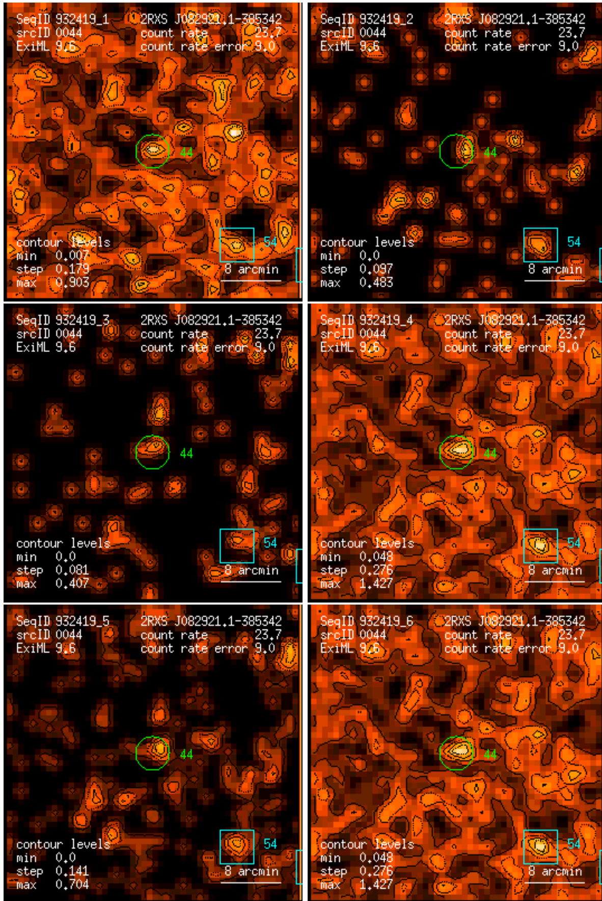
Figure 44: RASS 932419: detection 0044: band rate images, Gaussian filter: (1) PSPC channels 11 – 41, (2) 52 – 90, (3) 91 – 201, (4) 11 – 235, (5) 52 – 201, (6) 11 – 201. Broad band rates in counts/ks. Band rate contour levels in counts/ks/arcmin 2 .
