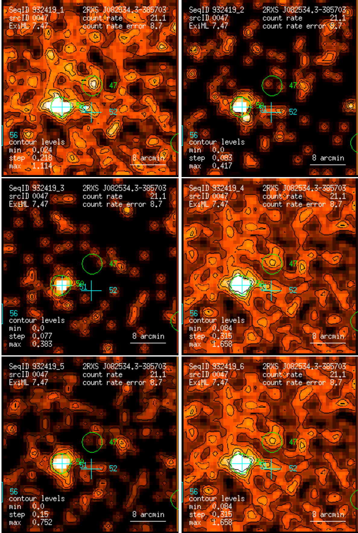
Figure 47: RASS 932419: detection 0047: band rate images, Gaussian filter: (1) PSPC channels 11 – 41, (2) 52 – 90, (3) 91 – 201, (4) 11 – 235, (5) 52 – 201, (6) 11 – 201. Broad band rates in counts/ks. Band rate contour levels in counts/ks/arcmin 2 .
