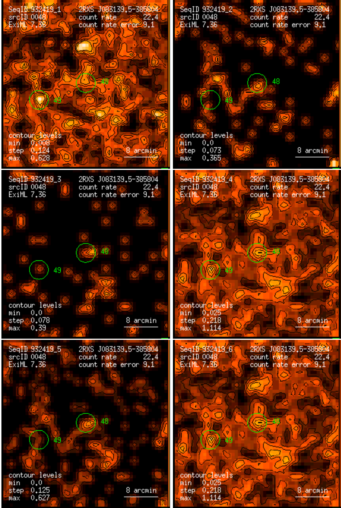
Figure 48: RASS 932419: detection 0048: band rate images, Gaussian filter: (1) PSPC channels 11 – 41, (2) 52 – 90, (3) 91 – 201, (4) 11 – 235, (5) 52 – 201, (6) 11 – 201. Broad band rates in counts/ks. Band rate contour levels in counts/ks/arcmin 2 .
