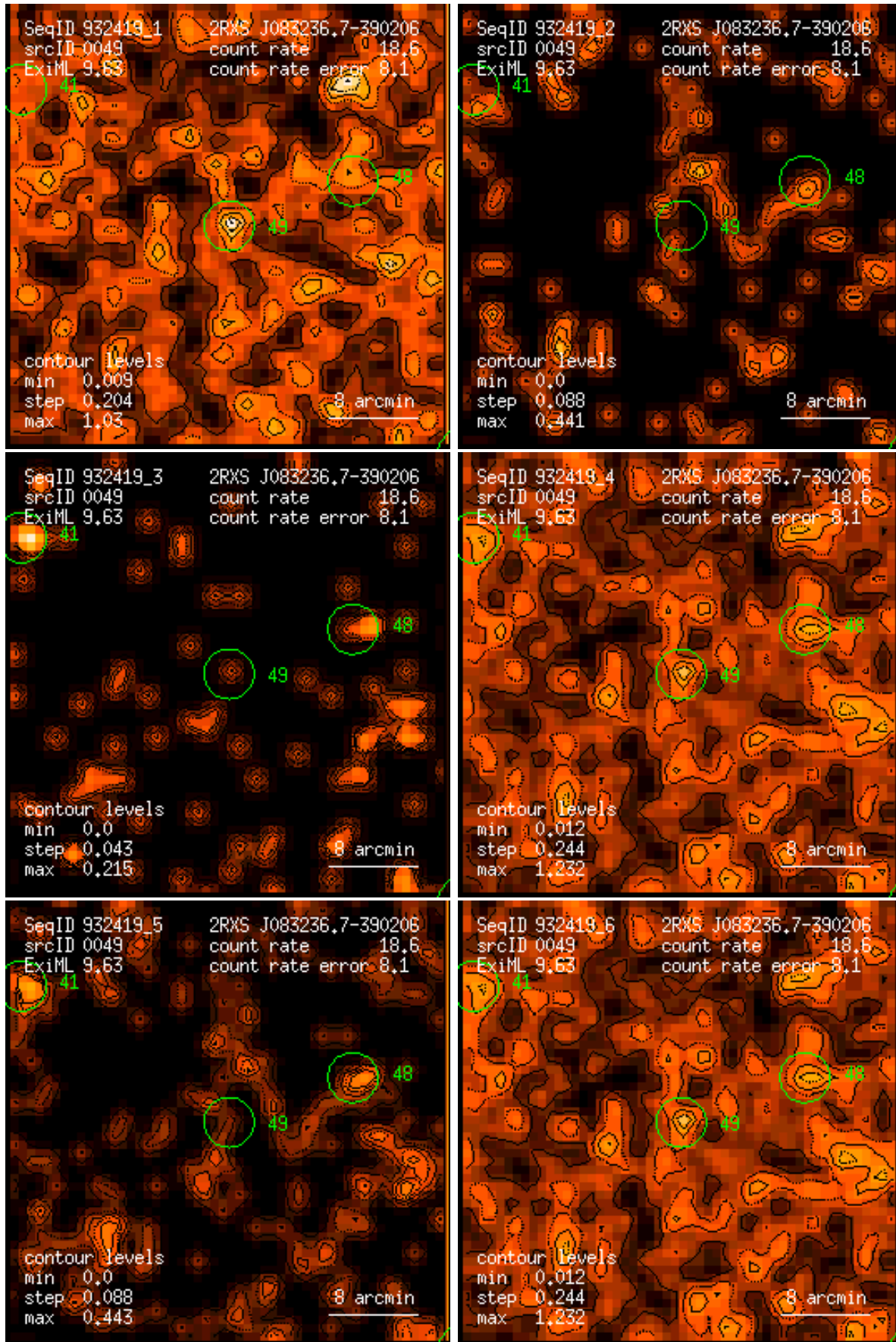
Figure 49: RASS 932419: detection 0049: band rate images, Gaussian filter: (1) PSPC channels 11 – 41, (2) 52 – 90, (3) 91 – 201, (4) 11 – 235, (5) 52 – 201, (6) 11 – 201. Broad band rates in counts/ks. Band rate contour levels in counts/ks/arcmin 2 .
