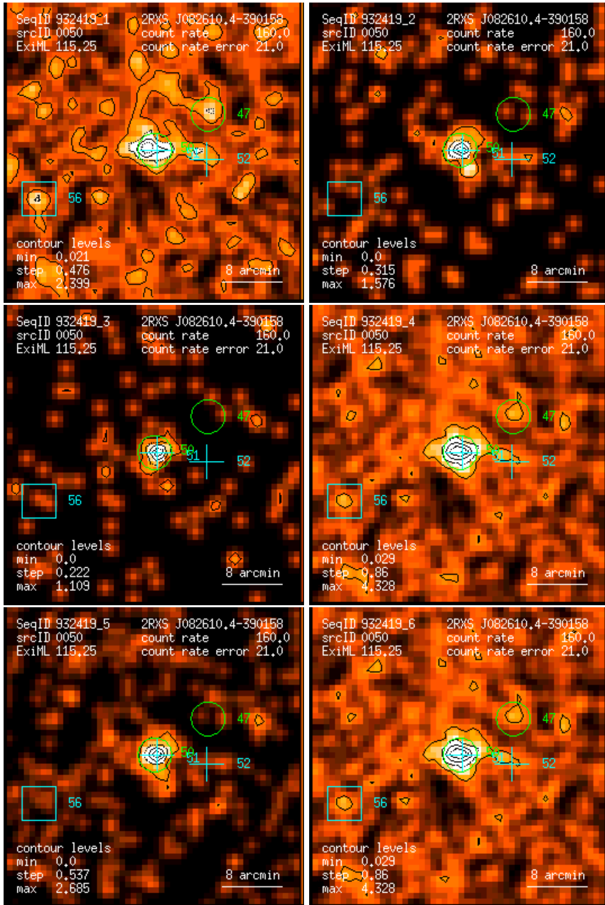
Figure 50: RASS 932419: detection 0050: band rate images, Gaussian filter: (1) PSPC channels 11 – 41, (2) 52 – 90, (3) 91 – 201, (4) 11 – 235, (5) 52 – 201, (6) 11 – 201. Broad band rates in counts/ks. Band rate contour levels in counts/ks/arcmin 2 .
