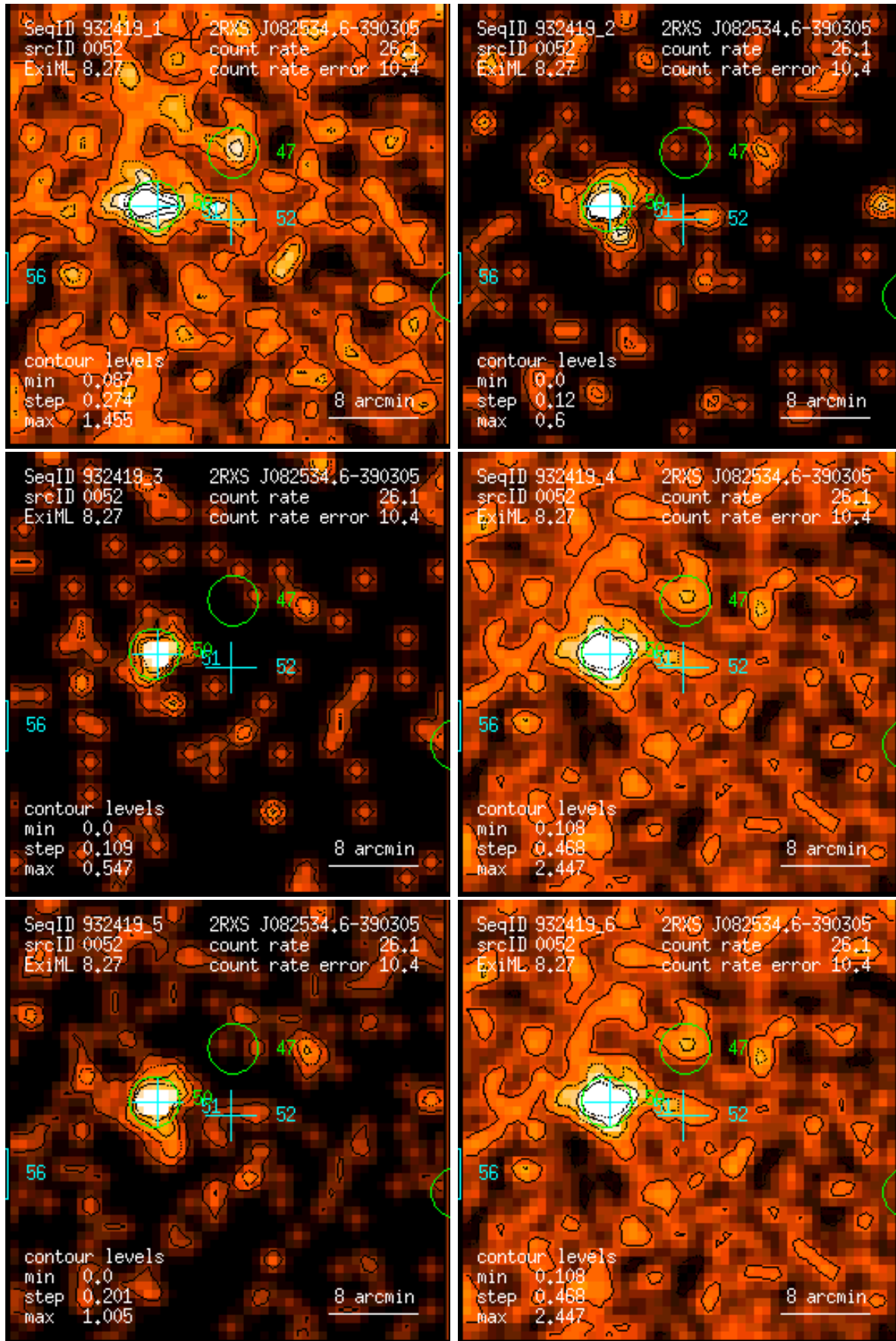
Figure 52: RASS 932419: detection 0052: band rate images, Gaussian filter: (1) PSPC channels 11 – 41, (2) 52 – 90, (3) 91 – 201, (4) 11 – 235, (5) 52 – 201, (6) 11 – 201. Broad band rates in counts/ks. Band rate contour levels in counts/ks/arcmin 2 .
