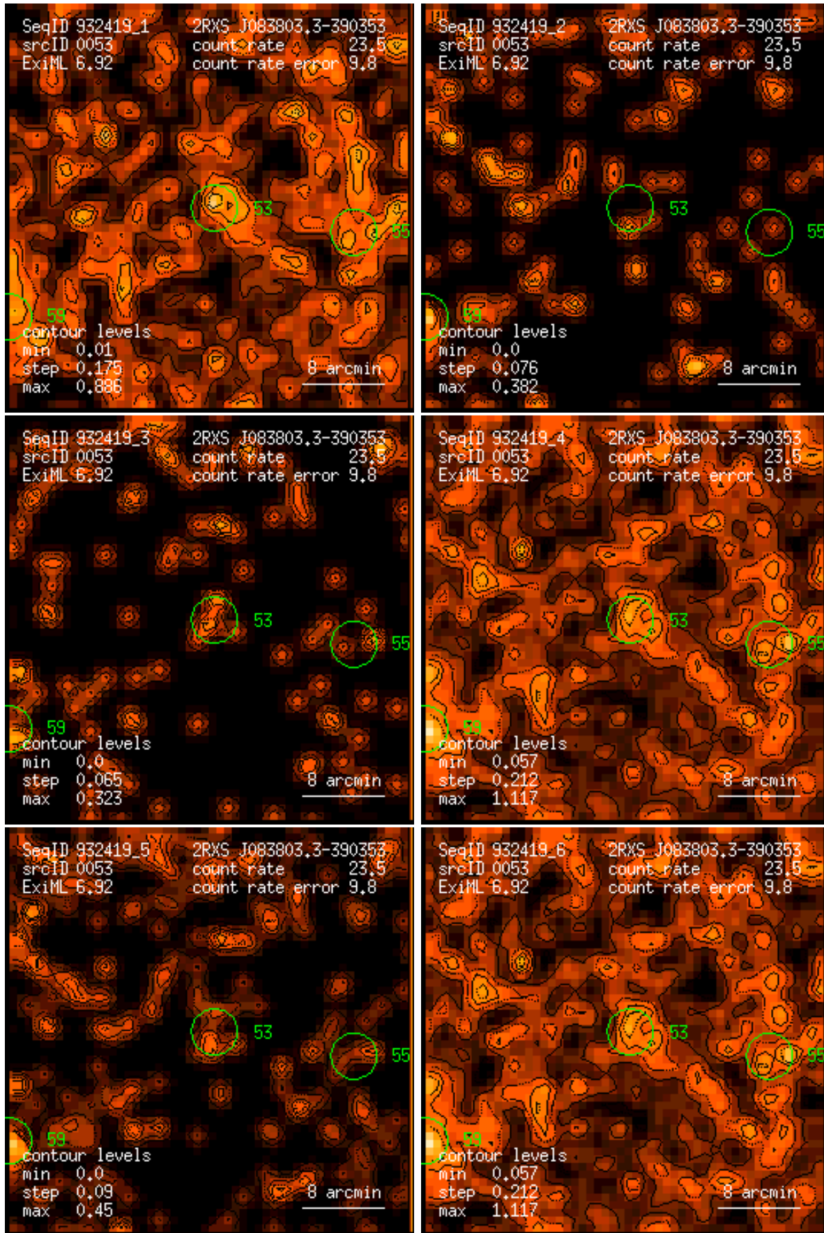
Figure 53: RASS 932419: detection 0053: band rate images, Gaussian filter: (1) PSPC channels 11 – 41, (2) 52 – 90, (3) 91 – 201, (4) 11 – 235, (5) 52 – 201, (6) 11 – 201. Broad band rates in counts/ks. Band rate contour levels in counts/ks/arcmin 2 .
