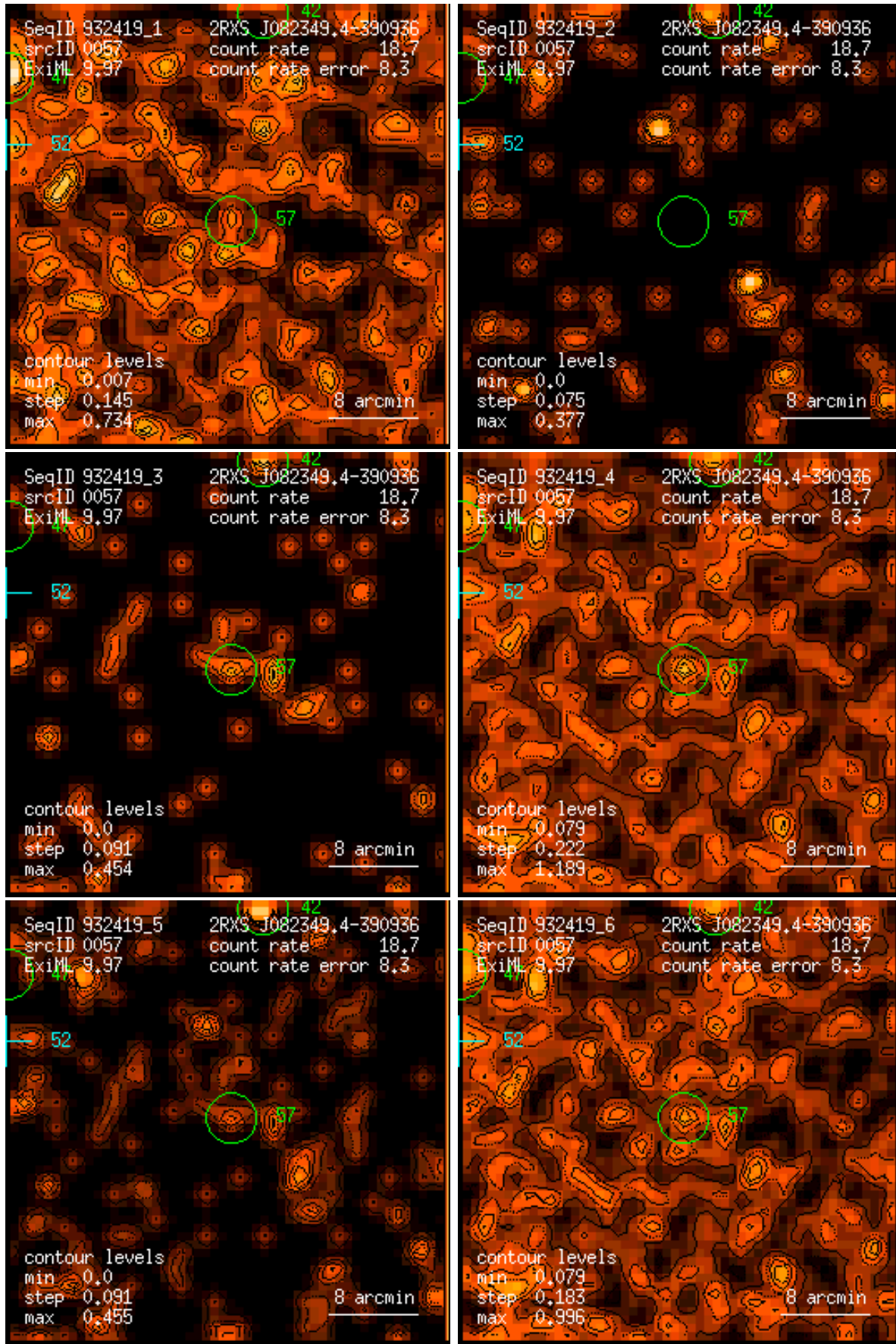
Figure 57: RASS 932419: detection 0057: band rate images, Gaussian filter: (1) PSPC channels 11 – 41, (2) 52 – 90, (3) 91 – 201, (4) 11 – 235, (5) 52 – 201, (6) 11 – 201. Broad band rates in counts/ks. Band rate contour levels in counts/ks/arcmin 2 .
