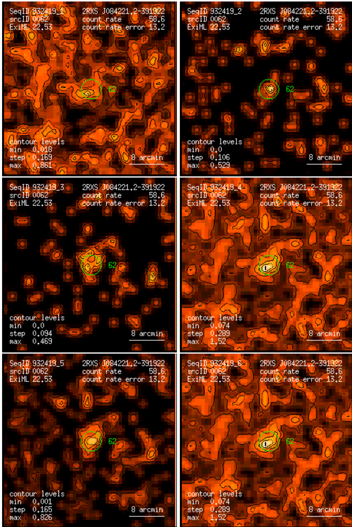
Figure 62: RASS 932419: detection 0062: band rate images, Gaussian filter: (1) PSPC channels 11 – 41, (2) 52 – 90, (3) 91 – 201, (4) 11 – 235, (5) 52 – 201, (6) 11 – 201. Broad band rates in counts/ks. Band rate contour levels in counts/ks/arcmin 2 .
