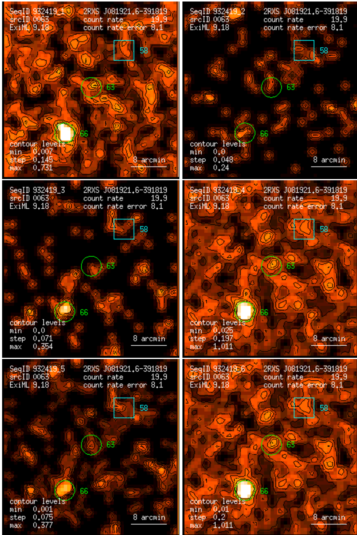
Figure 63: RASS 932419: detection 0063: band rate images, Gaussian filter: (1) PSPC channels 11 – 41, (2) 52 – 90, (3) 91 – 201, (4) 11 – 235, (5) 52 – 201, (6) 11 – 201. Broad band rates in counts/ks. Band rate contour levels in counts/ks/arcmin 2 .
