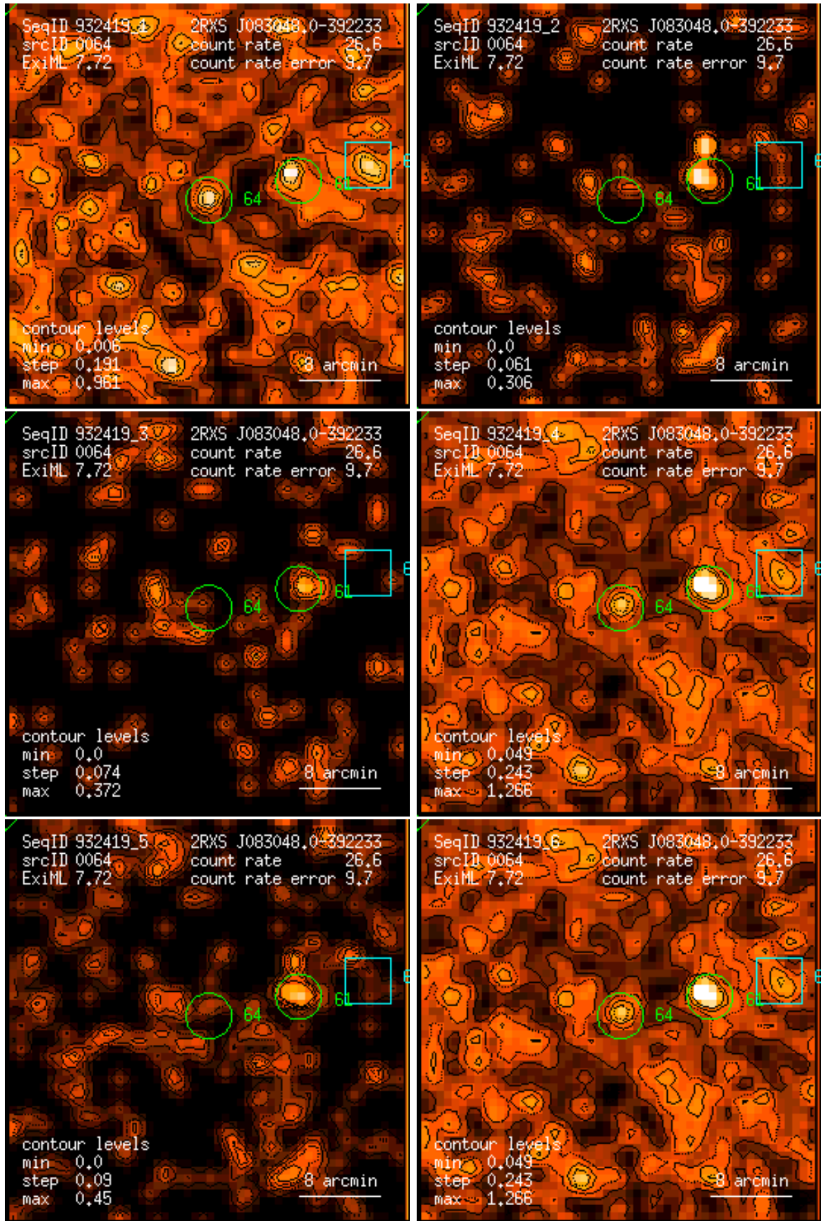
Figure 64: RASS 932419: detection 0064: band rate images, Gaussian filter: (1) PSPC channels 11 – 41, (2) 52 – 90, (3) 91 – 201, (4) 11 – 235, (5) 52 – 201, (6) 11 – 201. Broad band rates in counts/ks. Band rate contour levels in counts/ks/arcmin 2 .
