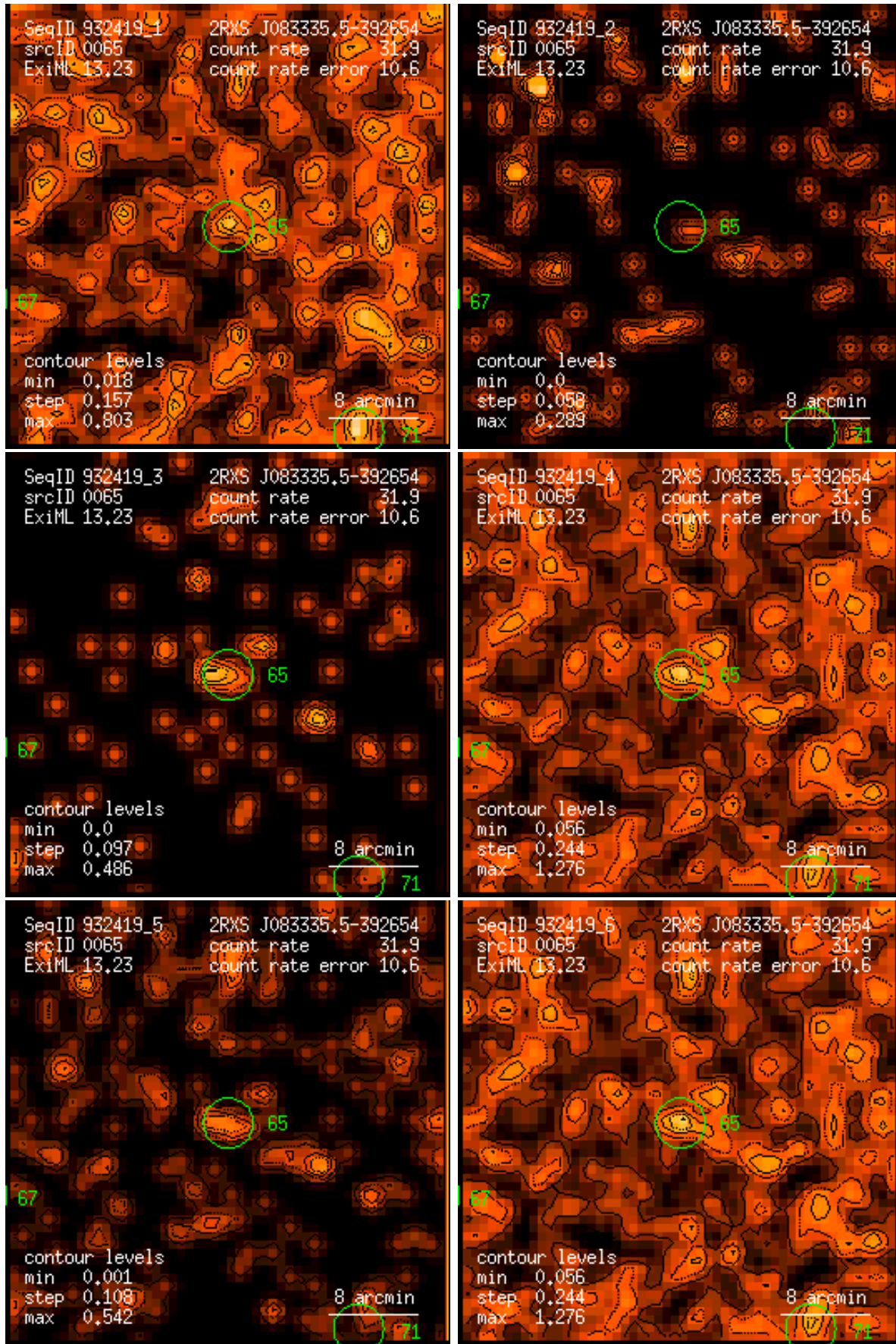
Figure 65: RASS 932419: detection 0065: band rate images, Gaussian filter: (1) PSPC channels 11 – 41, (2) 52 – 90, (3) 91 – 201, (4) 11 – 235, (5) 52 – 201, (6) 11 – 201. Broad band rates in counts/ks. Band rate contour levels in counts/ks/arcmin 2 .
