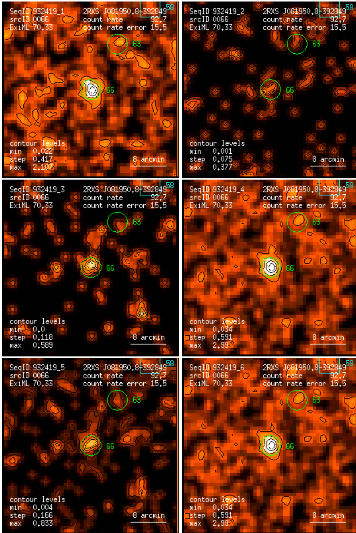
Figure 66: RASS 932419: detection 0066: band rate images, Gaussian filter: (1) PSPC channels 11 – 41, (2) 52 – 90, (3) 91 – 201, (4) 11 – 235, (5) 52 – 201, (6) 11 – 201. Broad band rates in counts/ks. Band rate contour levels in counts/ks/arcmin 2 .
