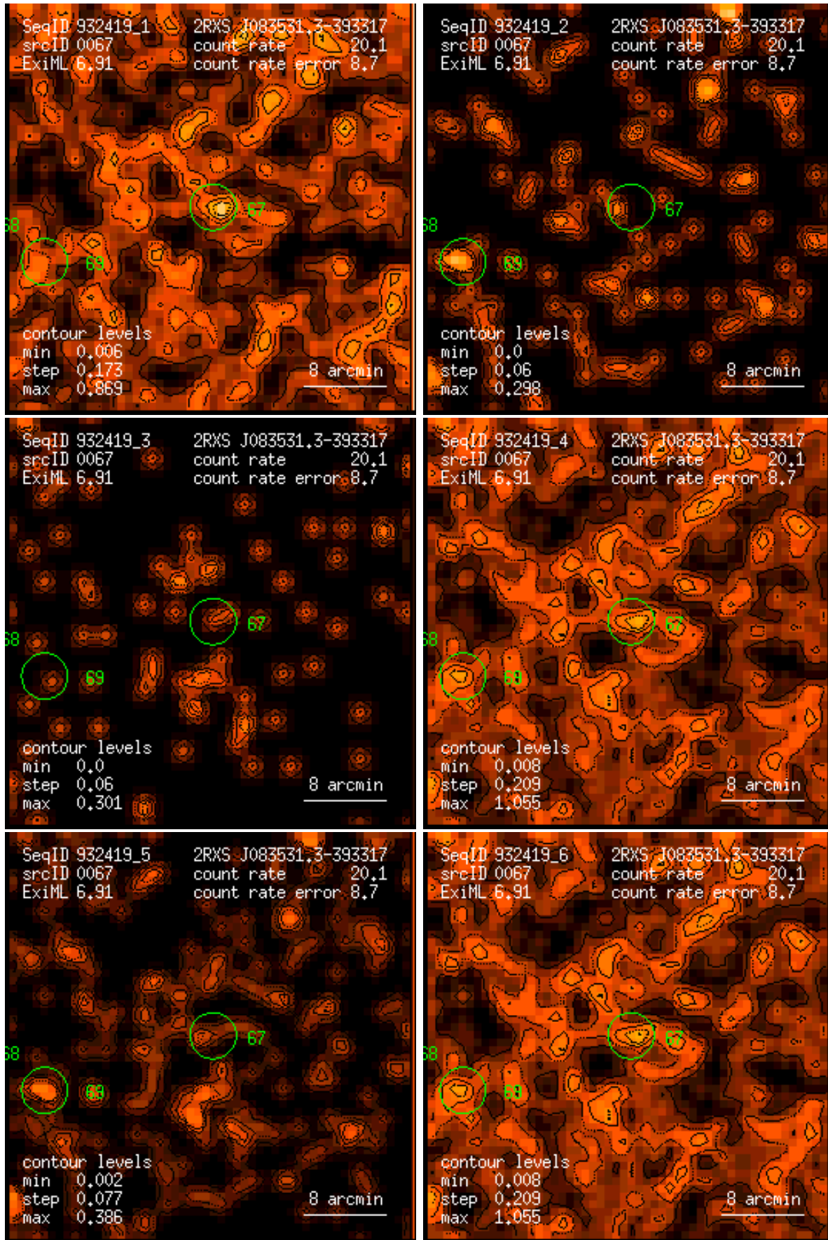
Figure 67: RASS 932419: detection 0067: band rate images, Gaussian filter: (1) PSPC channels 11 – 41, (2) 52 – 90, (3) 91 – 201, (4) 11 – 235, (5) 52 – 201, (6) 11 – 201. Broad band rates in counts/ks. Band rate contour levels in counts/ks/arcmin 2 .
