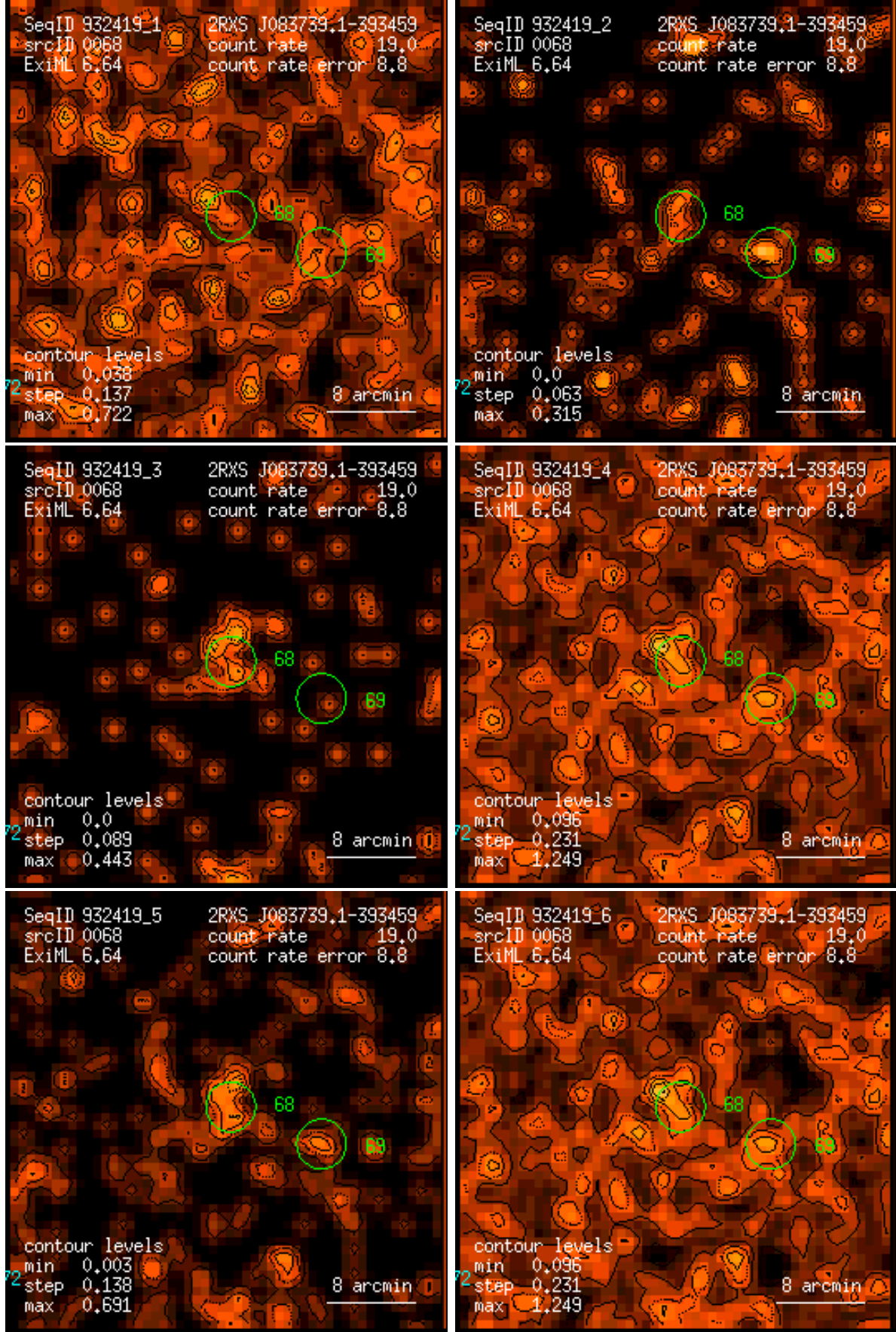
Figure 68: RASS 932419: detection 0068: band rate images, Gaussian filter: (1) PSPC channels 11 – 41, (2) 52 – 90, (3) 91 – 201, (4) 11 – 235, (5) 52 – 201, (6) 11 – 201. Broad band rates in counts/ks. Band rate contour levels in counts/ks/arcmin 2 .
