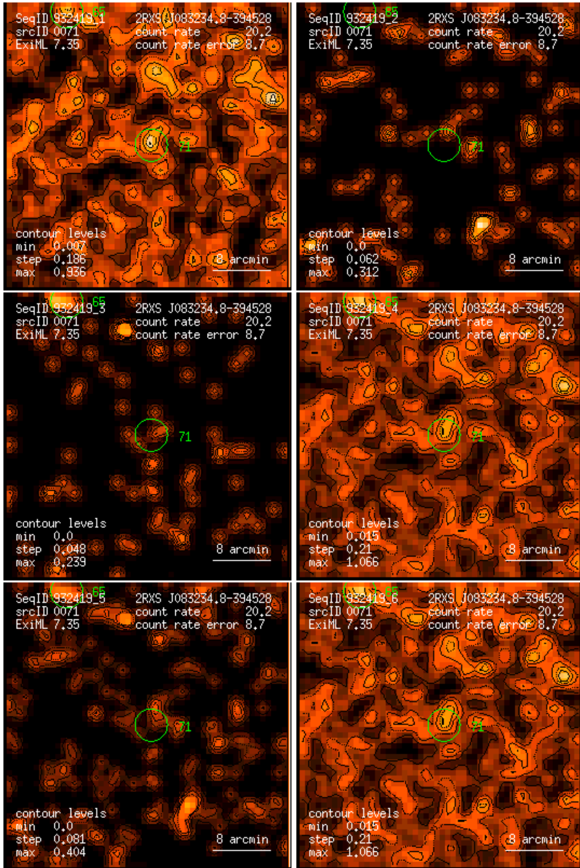
Figure 71: RASS 932419: detection 0071: band rate images, Gaussian filter: (1) PSPC channels 11 – 41, (2) 52 – 90, (3) 91 – 201, (4) 11 – 235, (5) 52 – 201, (6) 11 – 201. Broad band rates in counts/ks. Band rate contour levels in counts/ks/arcmin 2 .
