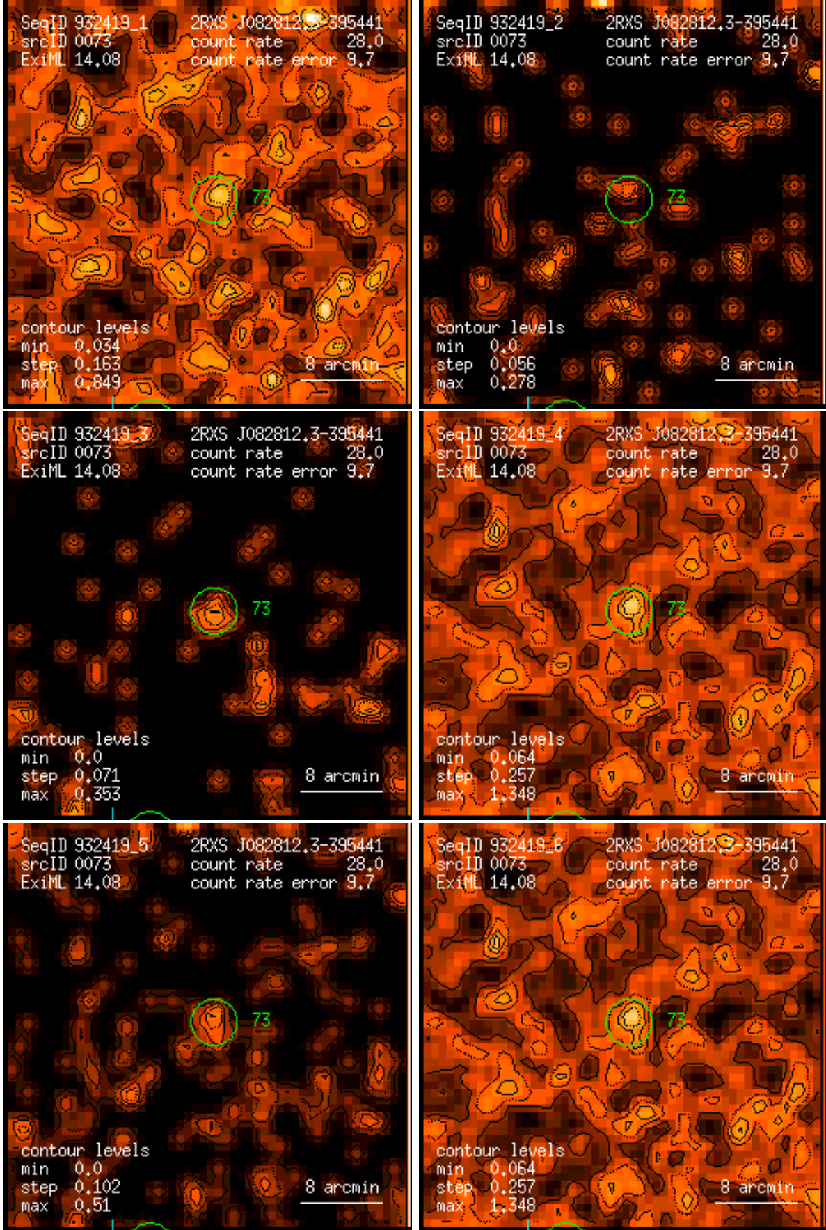
Figure 73: RASS 932419: detection 0073: band rate images, Gaussian filter: (1) PSPC channels 11 – 41, (2) 52 – 90, (3) 91 – 201, (4) 11 – 235, (5) 52 – 201, (6) 11 – 201. Broad band rates in counts/ks. Band rate contour levels in counts/ks/arcmin 2 .
