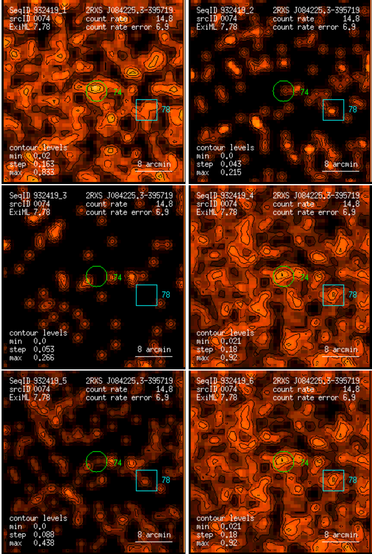
Figure 74: RASS 932419: detection 0074: band rate images, Gaussian filter: (1) PSPC channels 11 – 41, (2) 52 – 90, (3) 91 – 201, (4) 11 – 235, (5) 52 – 201, (6) 11 – 201. Broad band rates in counts/ks. Band rate contour levels in counts/ks/arcmin 2 .
