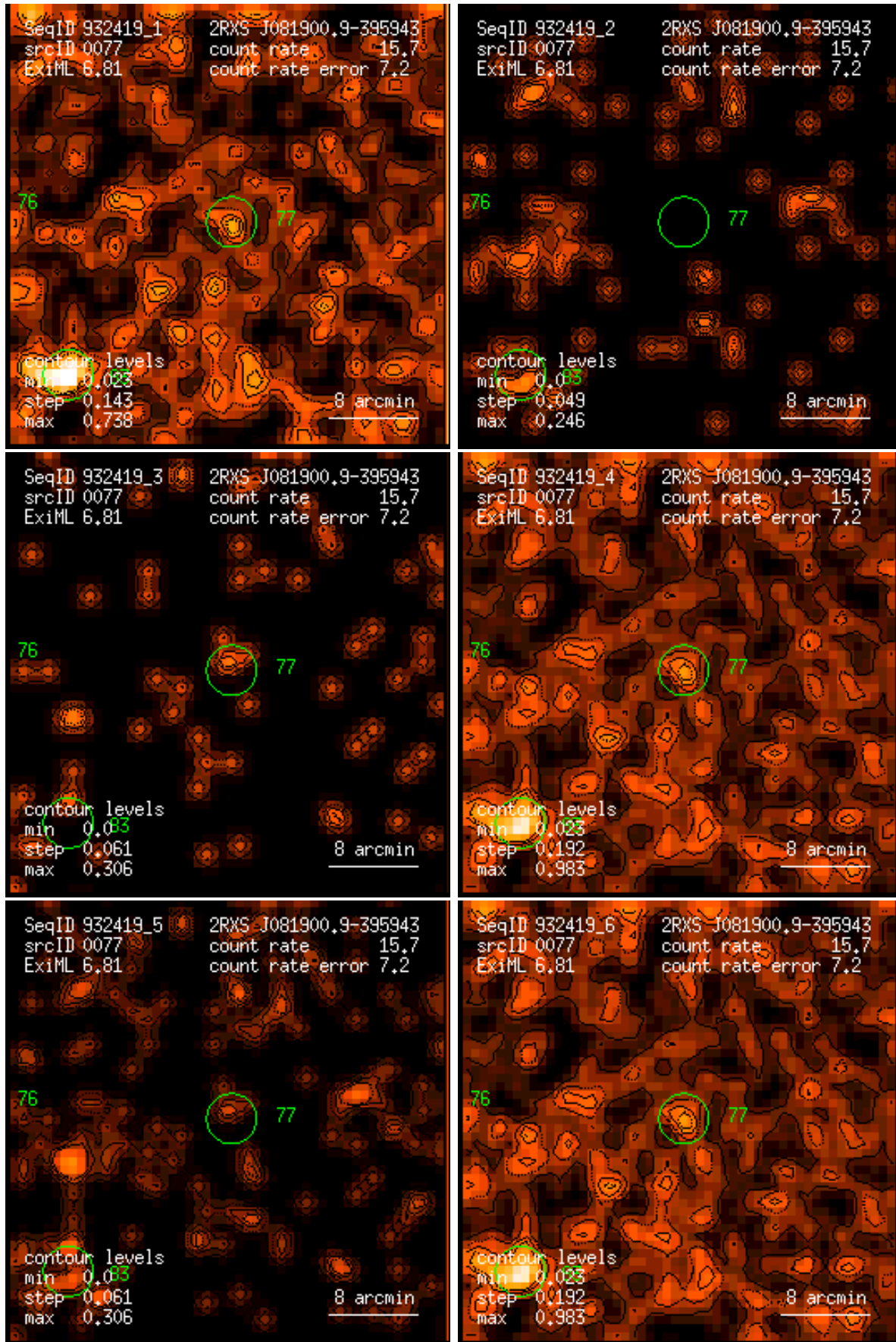
Figure 77: RASS 932419: detection 0077: band rate images, Gaussian filter: (1) PSPC channels 11 – 41, (2) 52 – 90, (3) 91 – 201, (4) 11 – 235, (5) 52 – 201, (6) 11 – 201. Broad band rates in counts/ks. Band rate contour levels in counts/ks/arcmin 2 .
